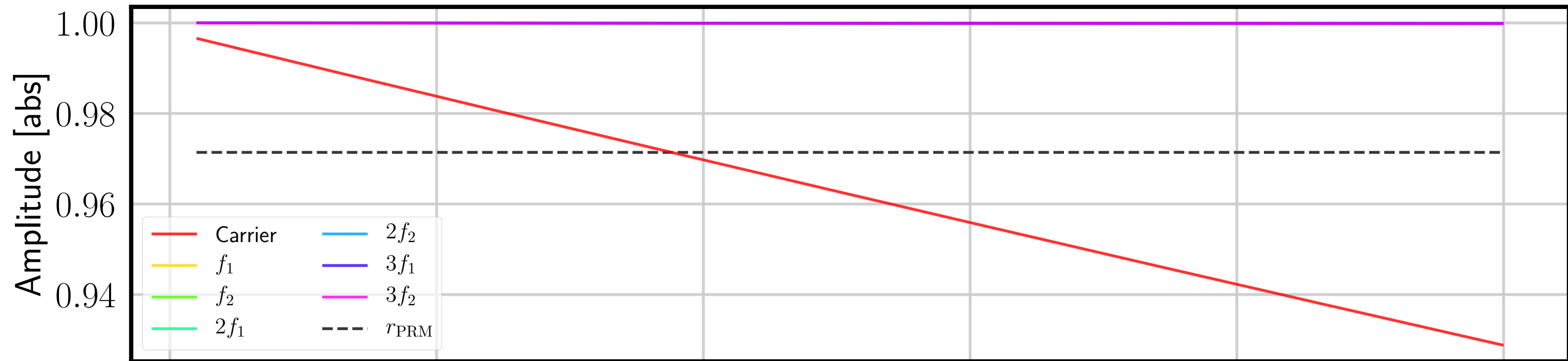
Analytic (amplitude) reflectivity of arm cavity for various fields
