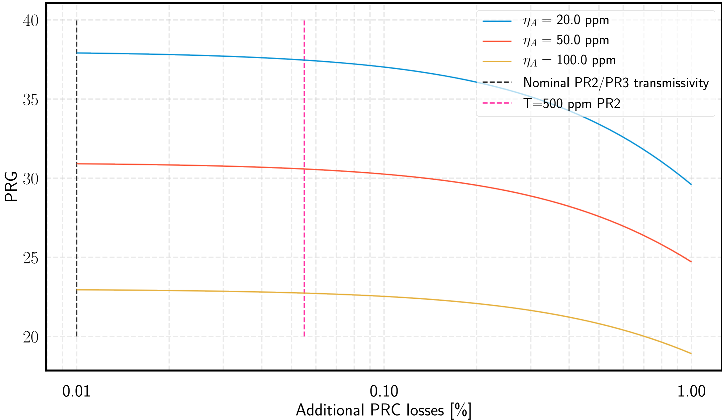
Relative importance of losses in the arm cavity and PRC for recycling gain (assuming fixed MM loss of 0.5 %)
