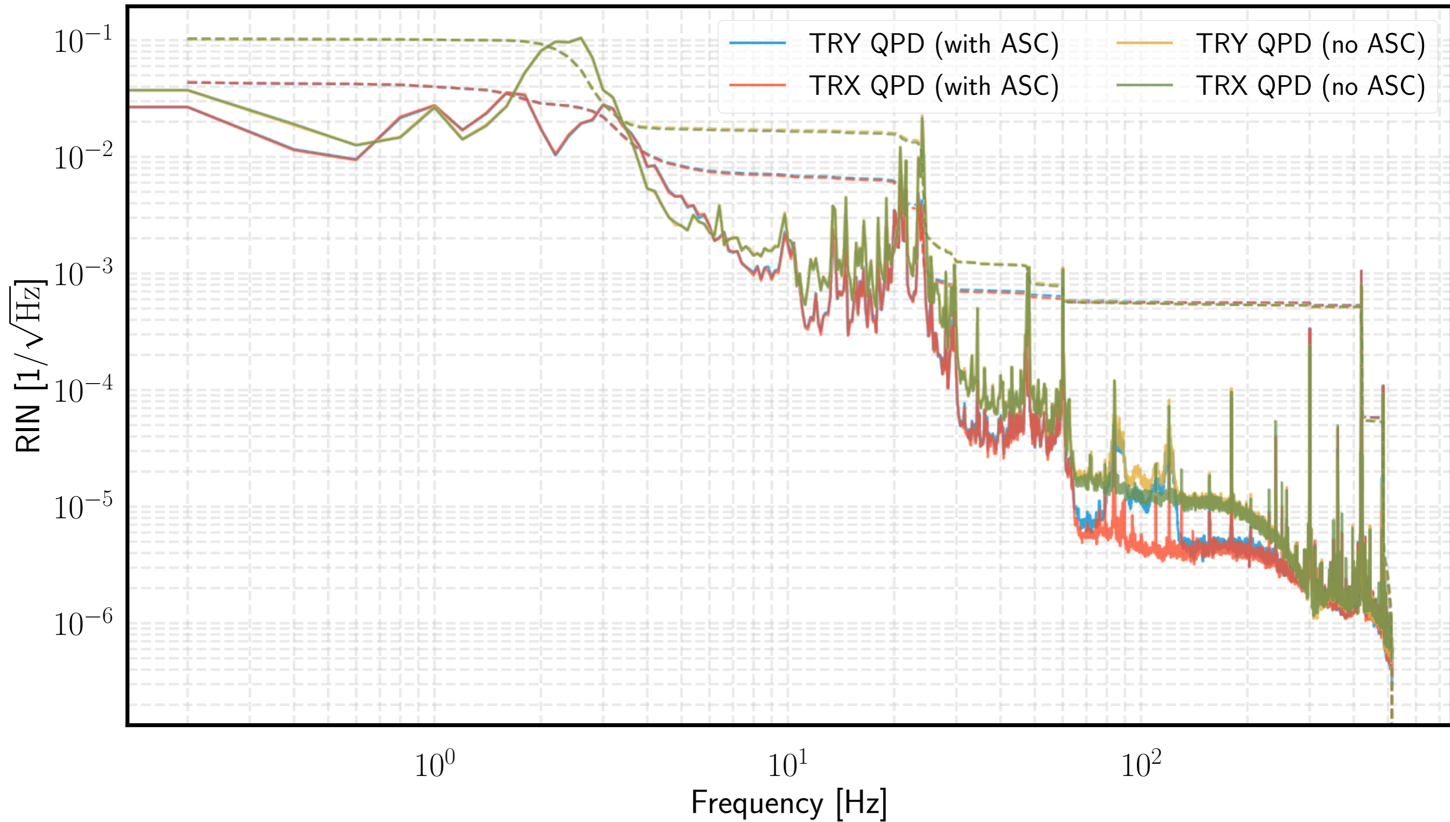
Arm transmission RIN for single arm lock vs PRFPMI with and without PRC ASC
