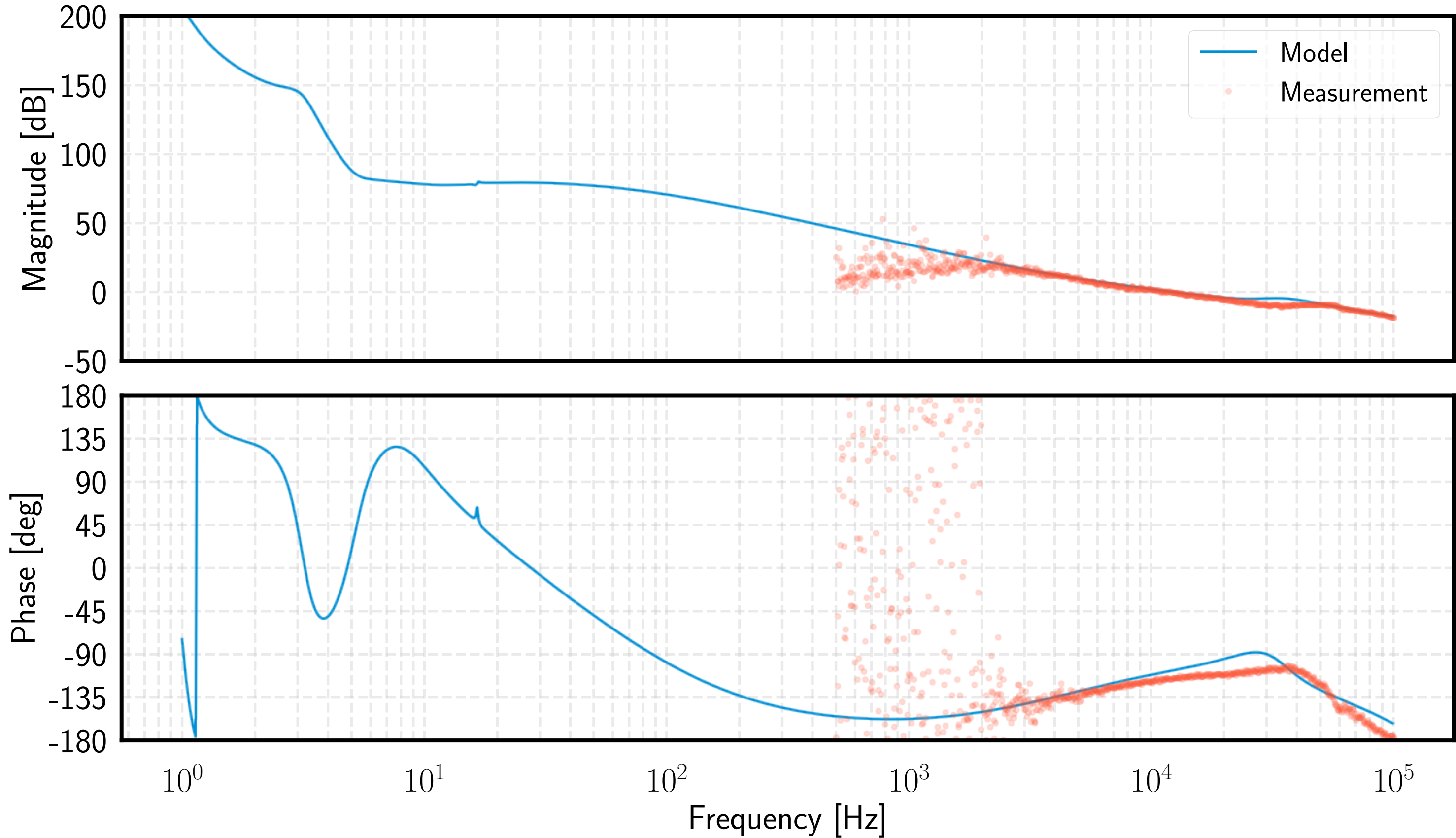
CARM OLTF model and measurement
