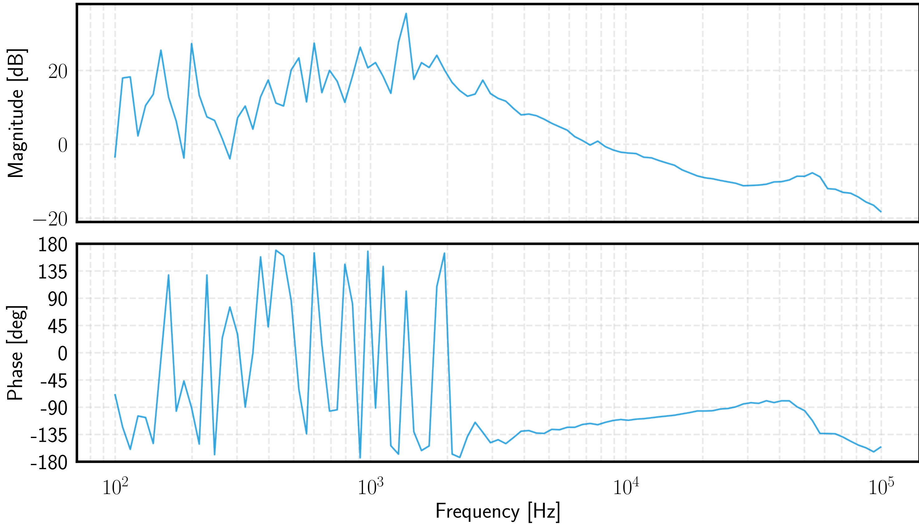
40m PRFPMI CARM OLTF measurement, 24 May 2020
