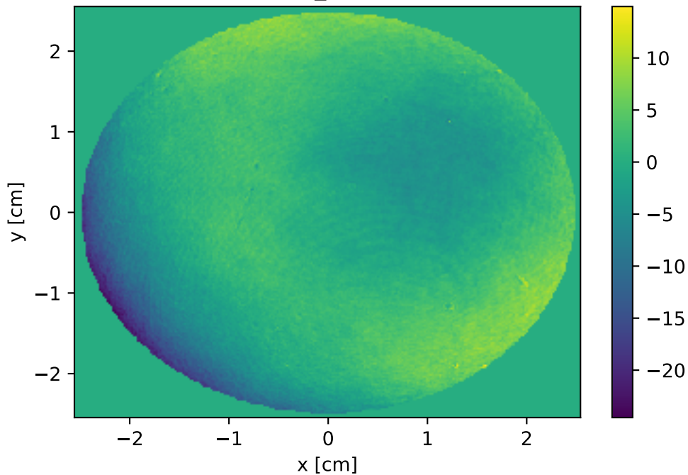
Surface map ETM_x, type phase both
