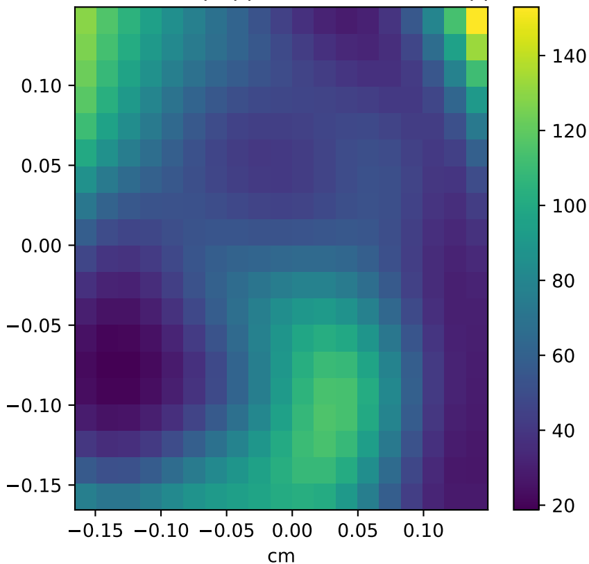
ETMX Loss Map (ppm). Mean = 61.67 ppm
