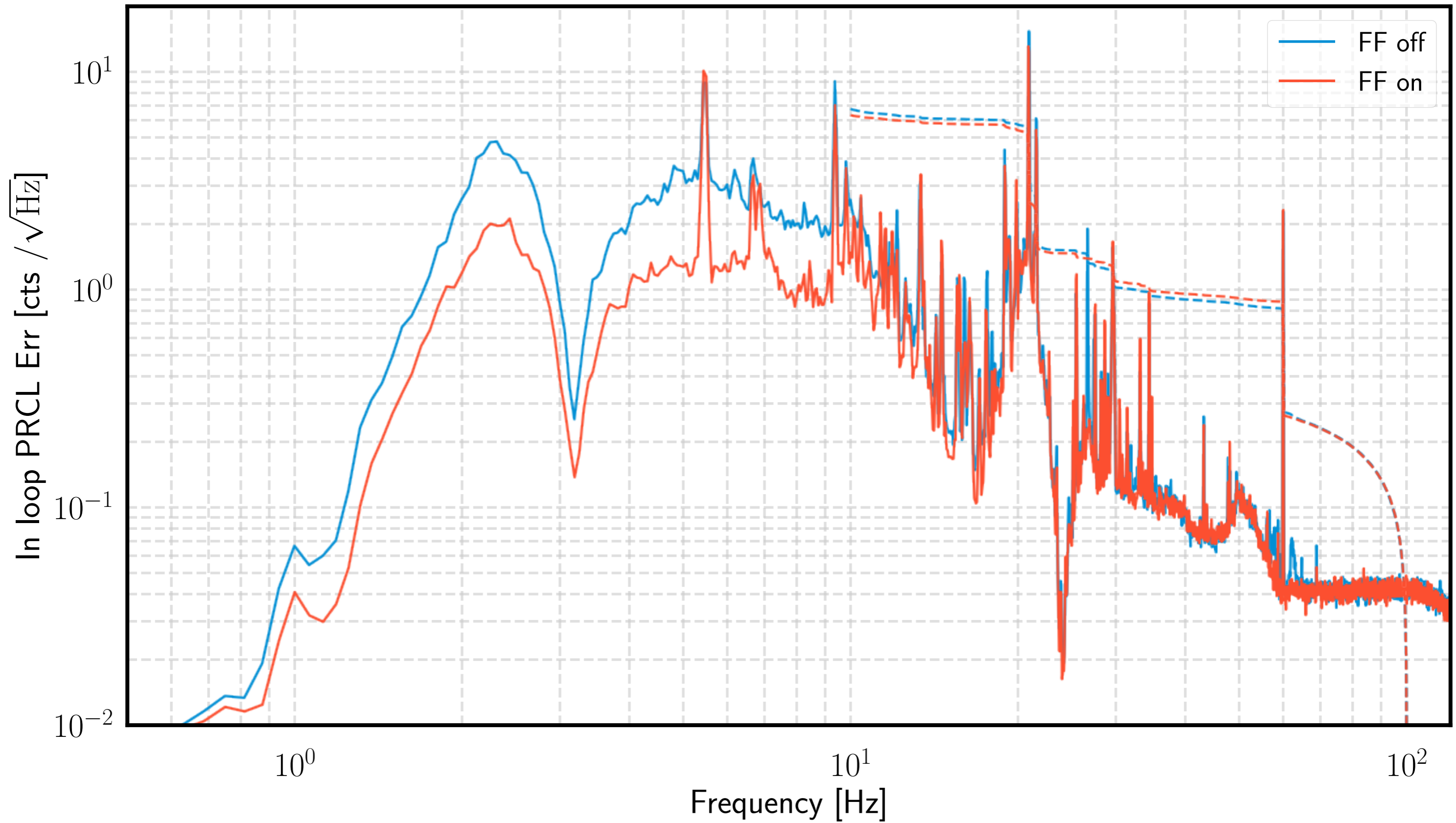
Effect of POP angular feedforward on PRCL length
