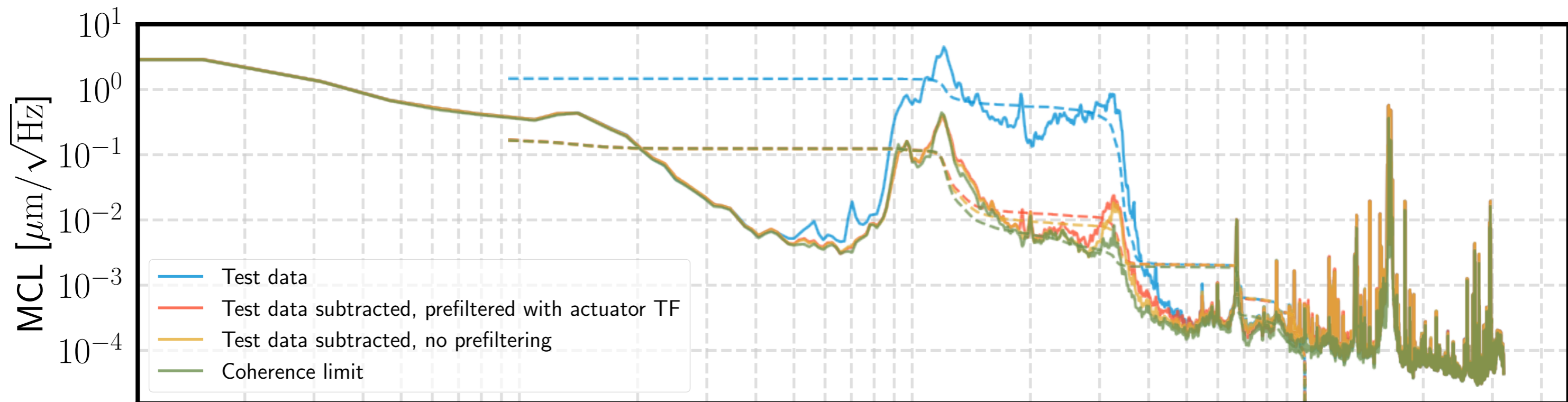
IMC length stabilization with seismic feedforward (offline, FIR)
