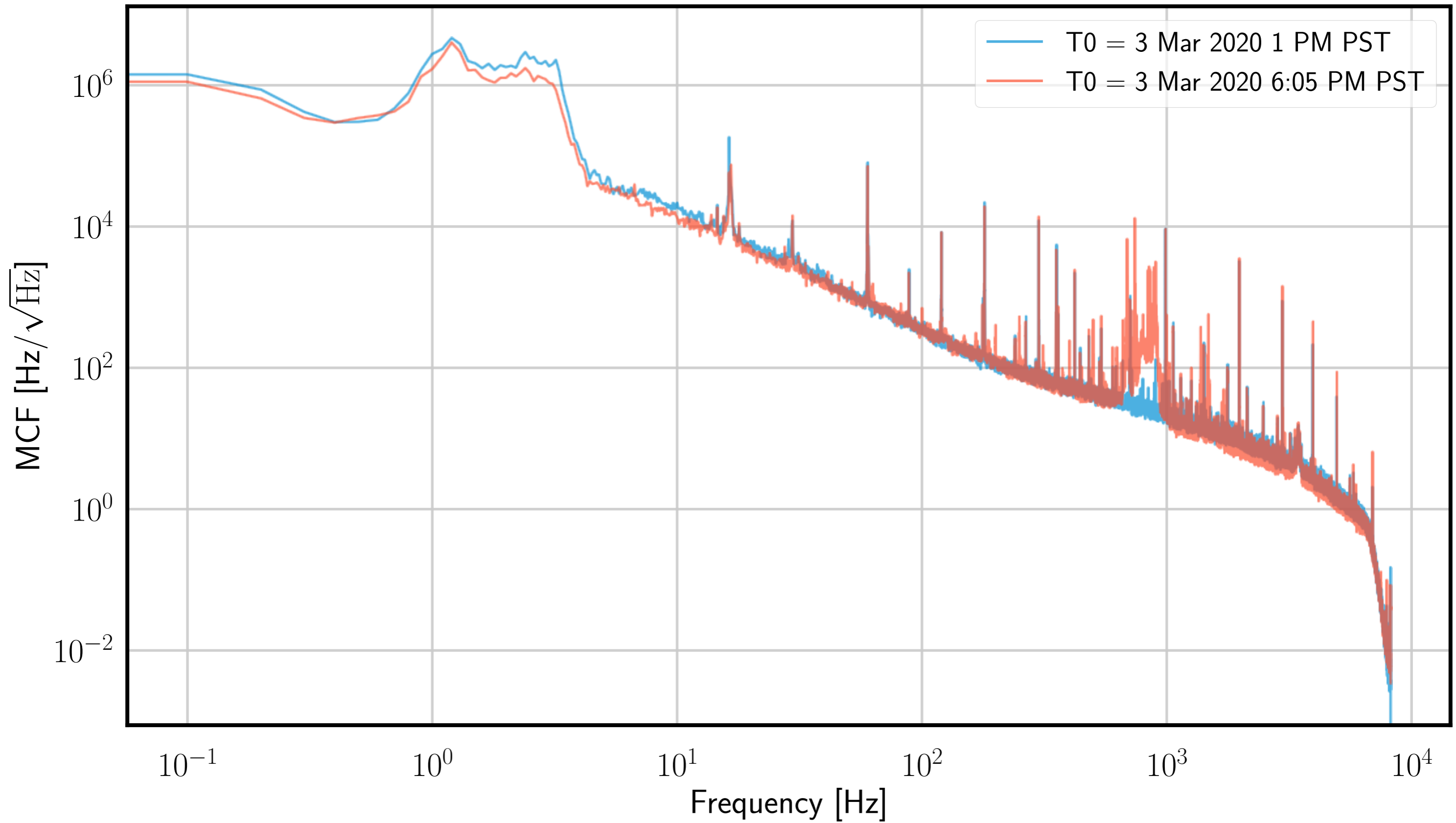
MCF frequency noise
