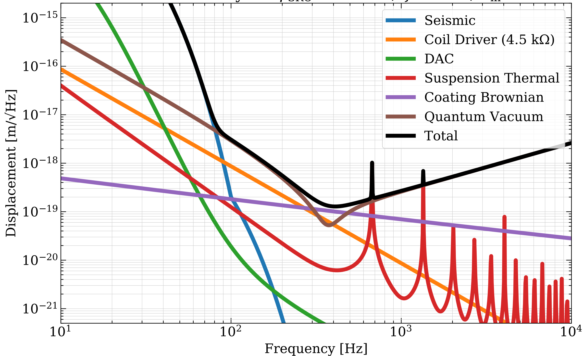
40m DARM sensitivity for \phi_{\text{SRC}} = -0.01^\circ , \zeta = 88.0^\circ , P_{\text{in}} = 20 \text{ W}
