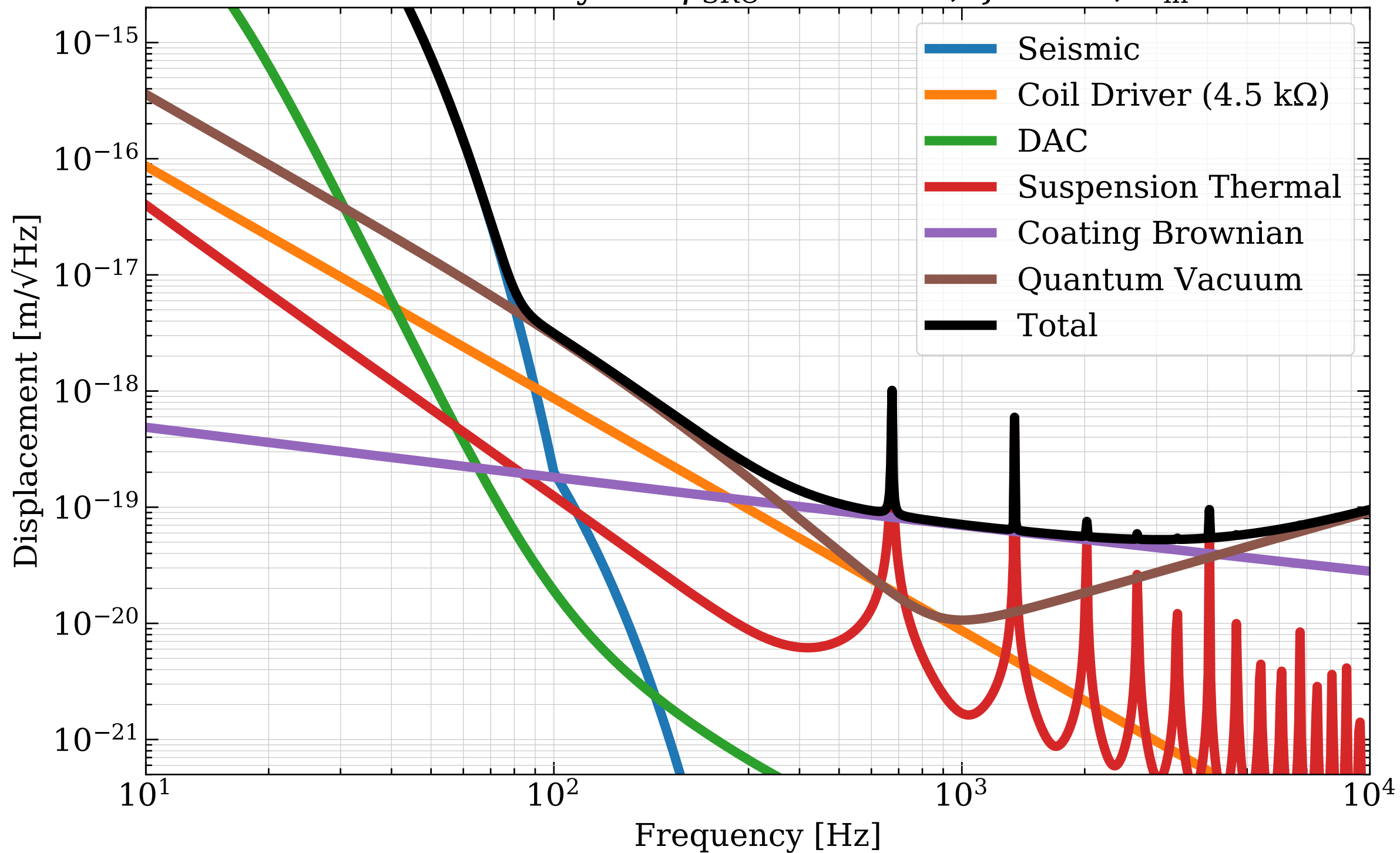
40m DARM sensitivity for \phi_{\text{SRC}} = -0.01^\circ , \zeta = 0.0^\circ , P_{\text{in}} = 20 \text{ W}
