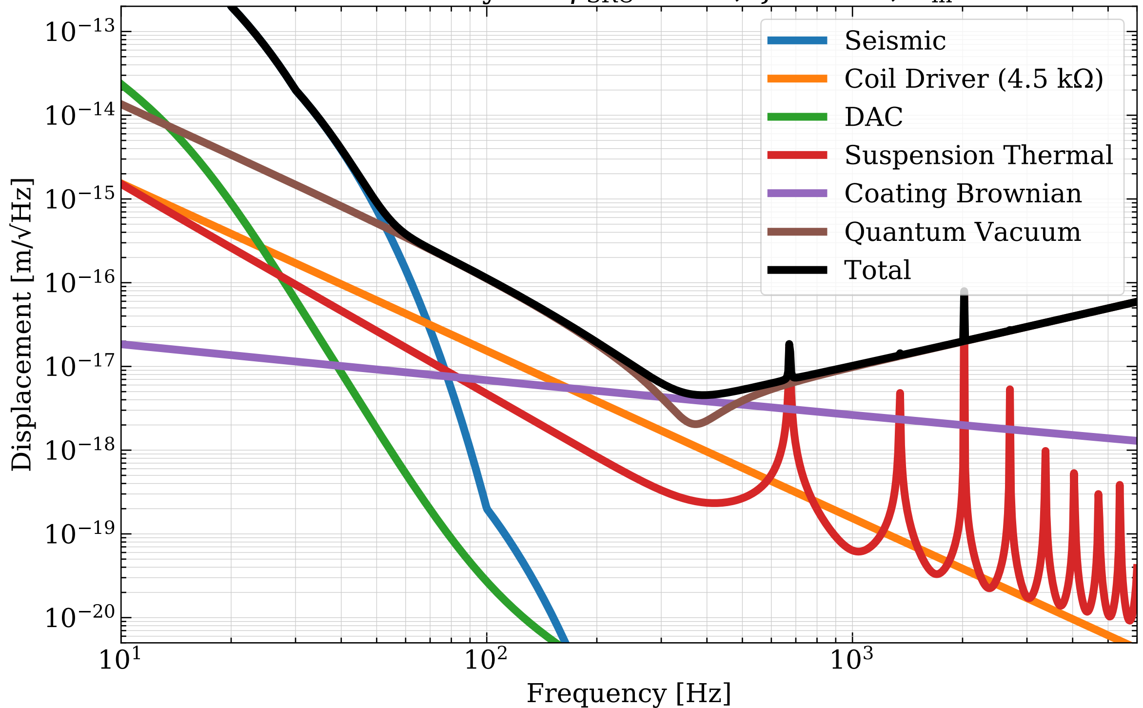
40m DARM sensitivity for \phi_{\text{SRC}} = 0.0^\circ , \zeta = 88.0^\circ , P_{\text{in}} = 20.0 \text{ W}
