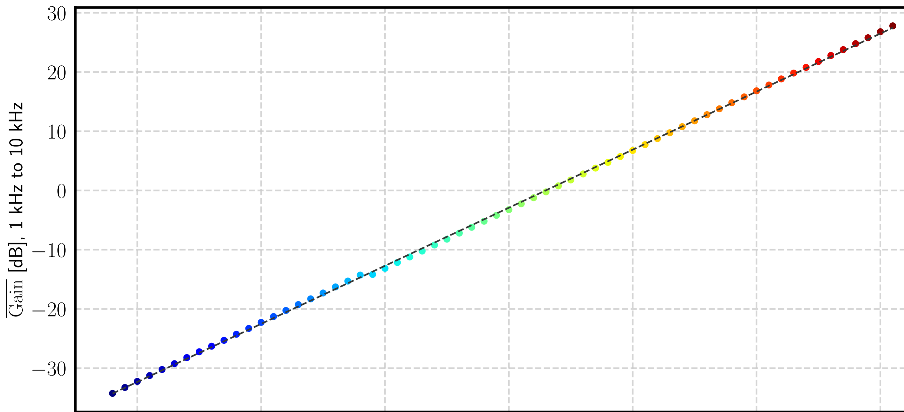
IMC Servo board AO path gain slider calibration
