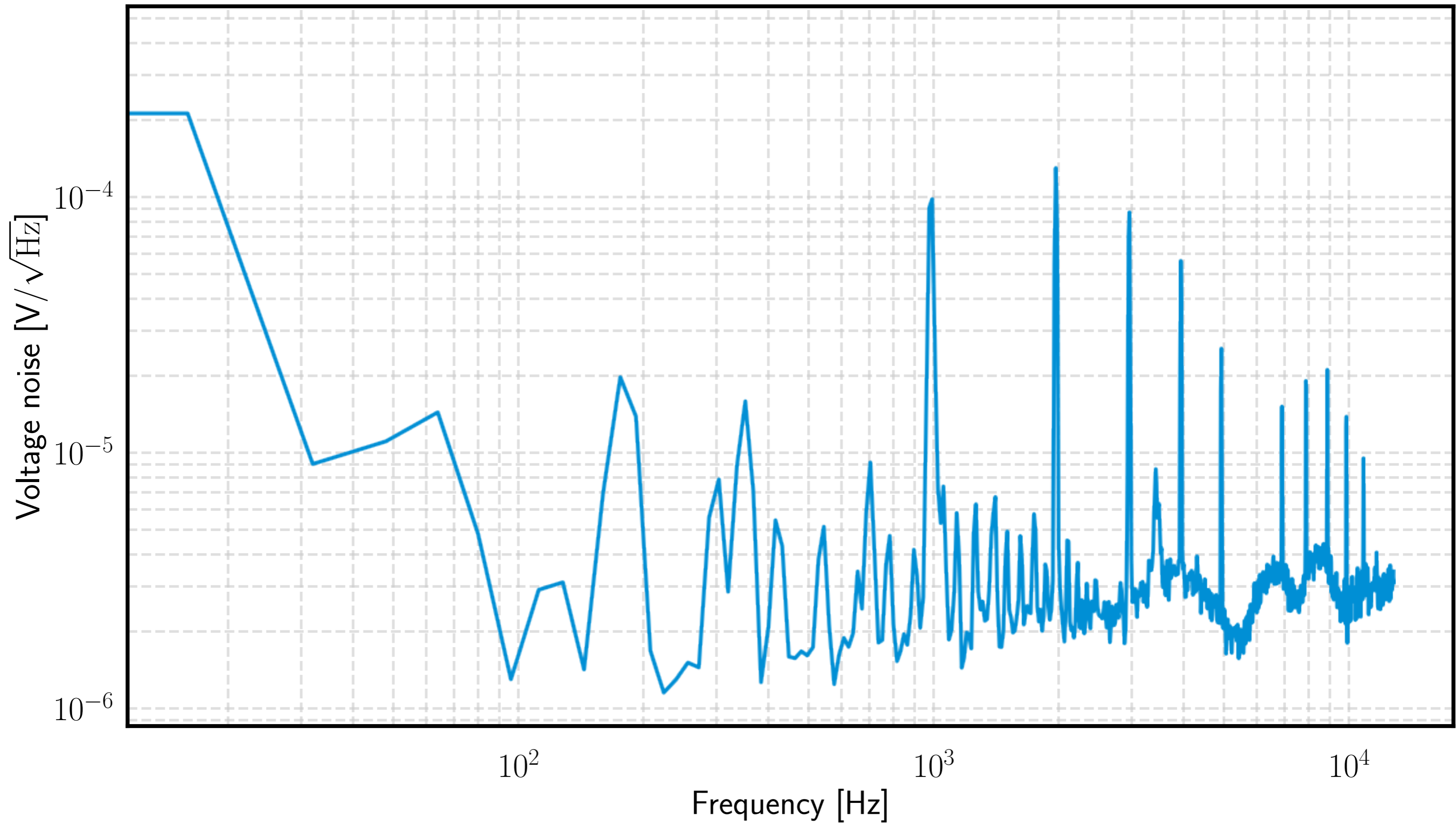
IMC in loop noise, measured at TP1A
