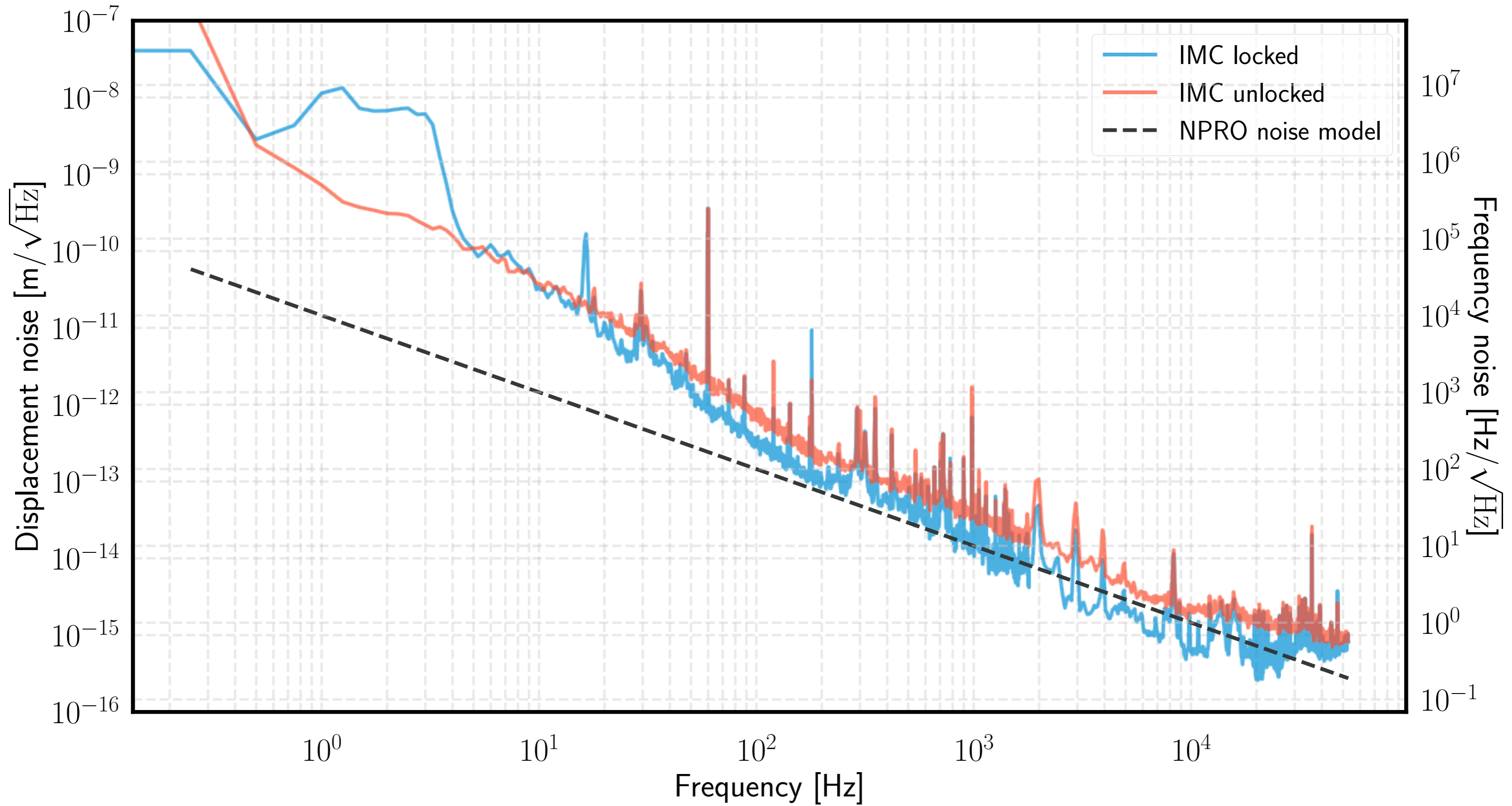
PMC as a frequency noise analyzer
