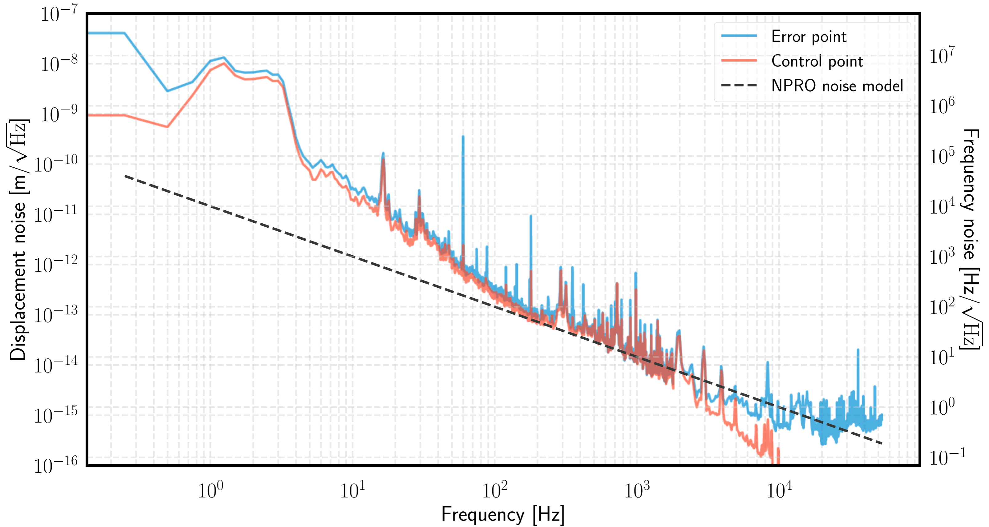
PMC displacement noise estimate, 24 Jan 2020
