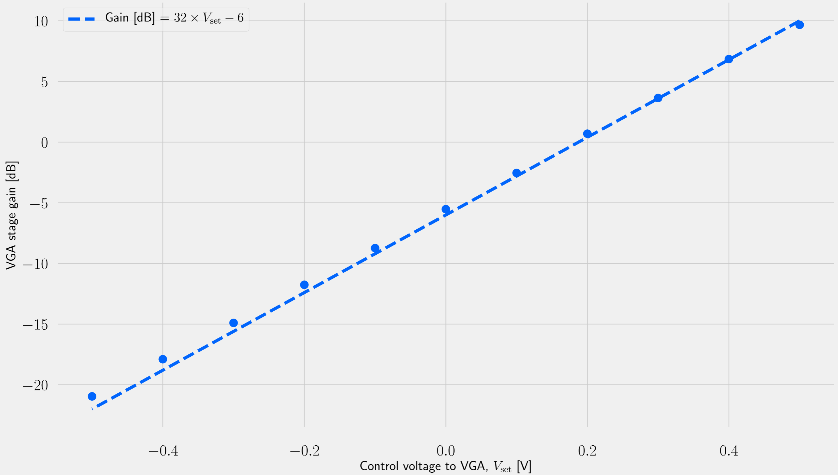
VGA gain linearity after IC replacement
