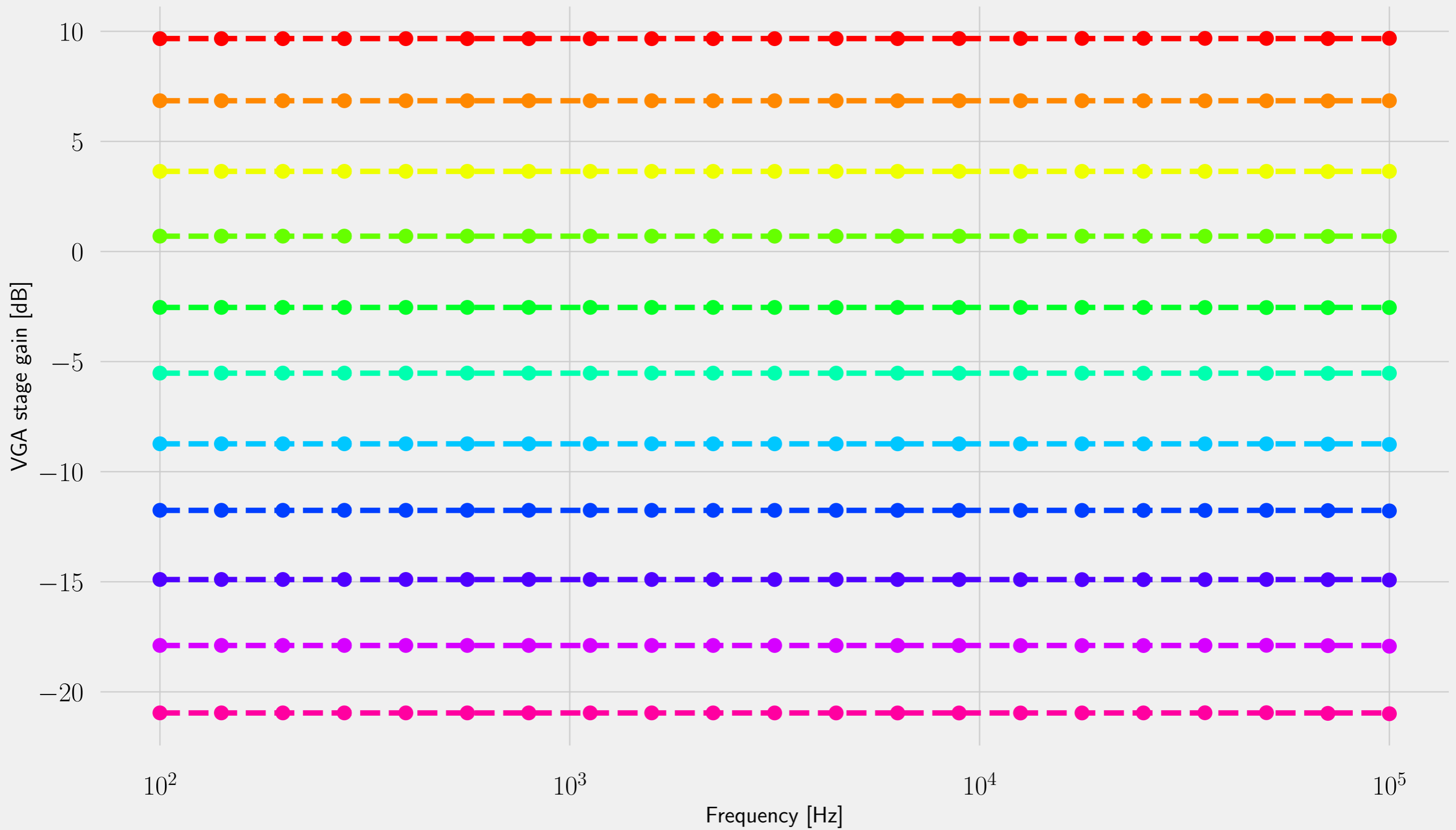
PMC Servo VGA stage gain after IC replacement
