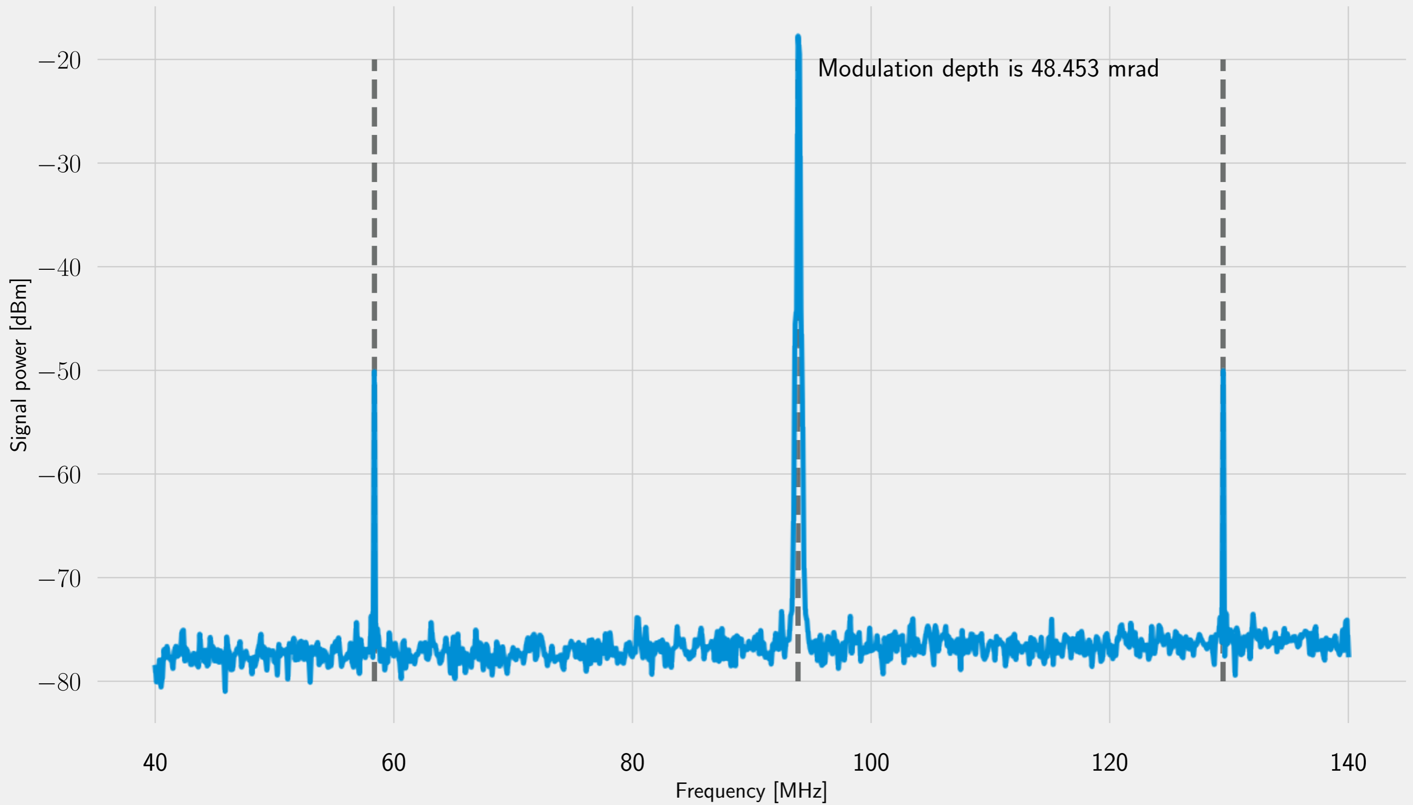
PMC servo modulation depth estimation
