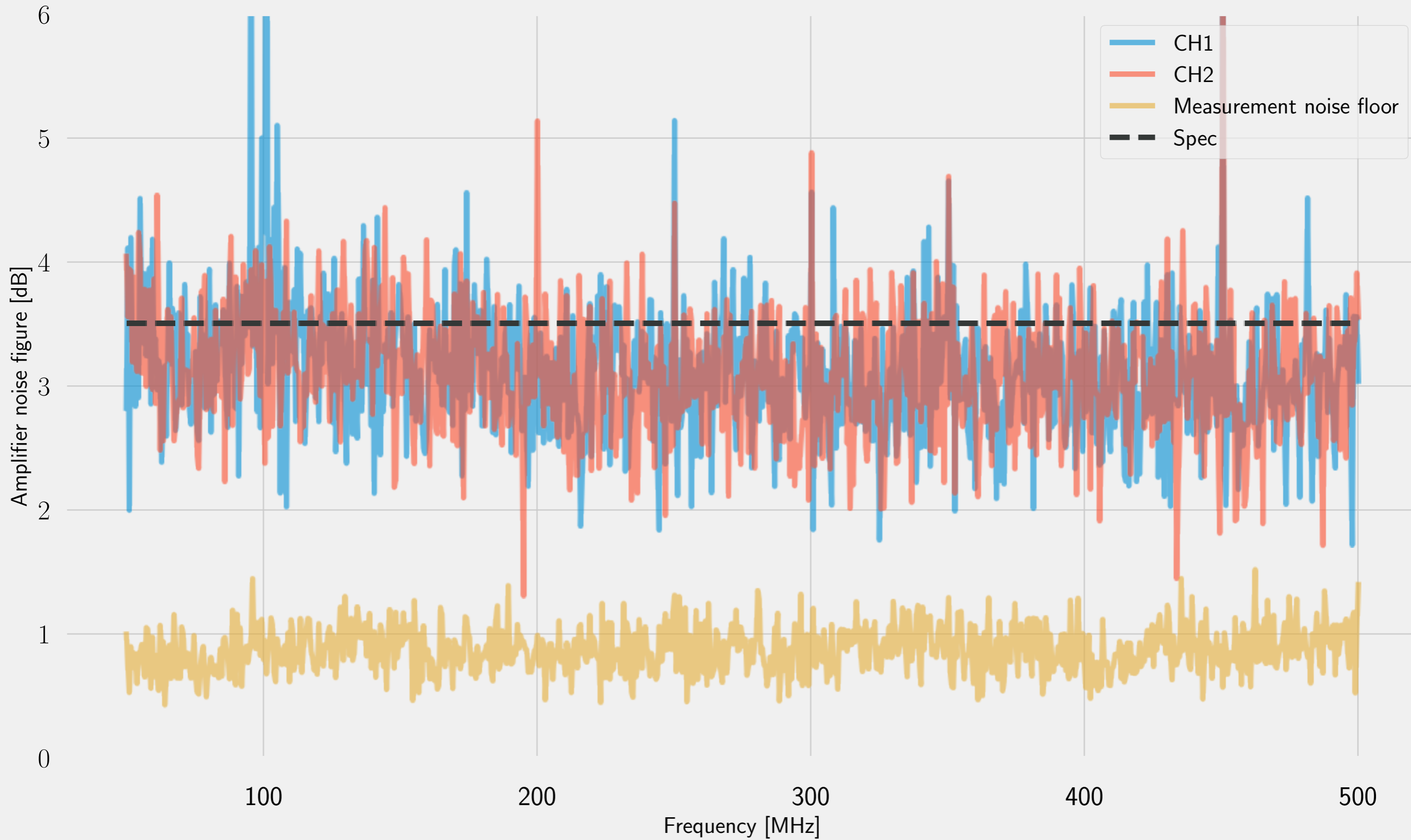
Measurement of noise of ZHL-1010+
