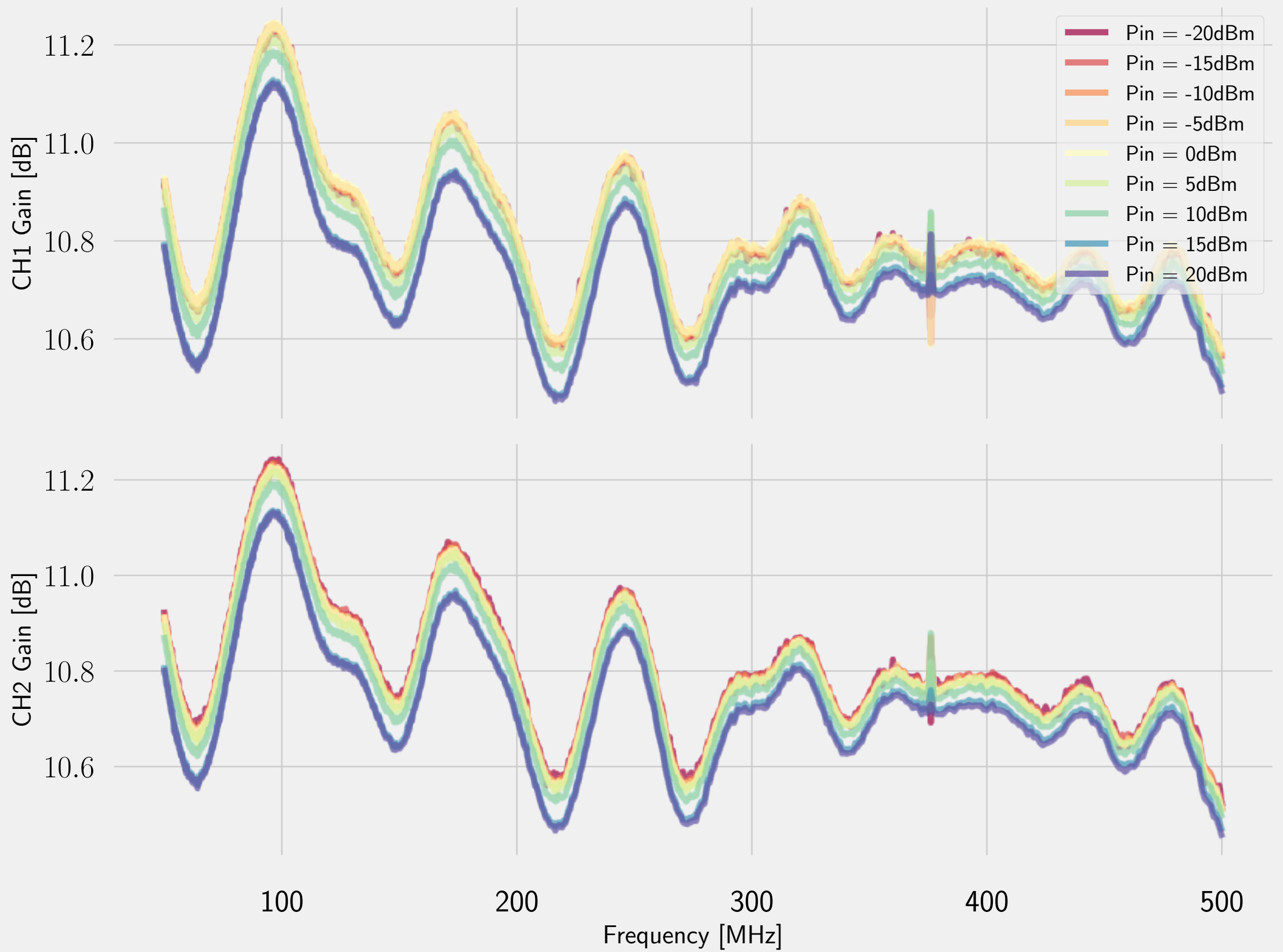
Measurement of gain of ZHL-1010+
