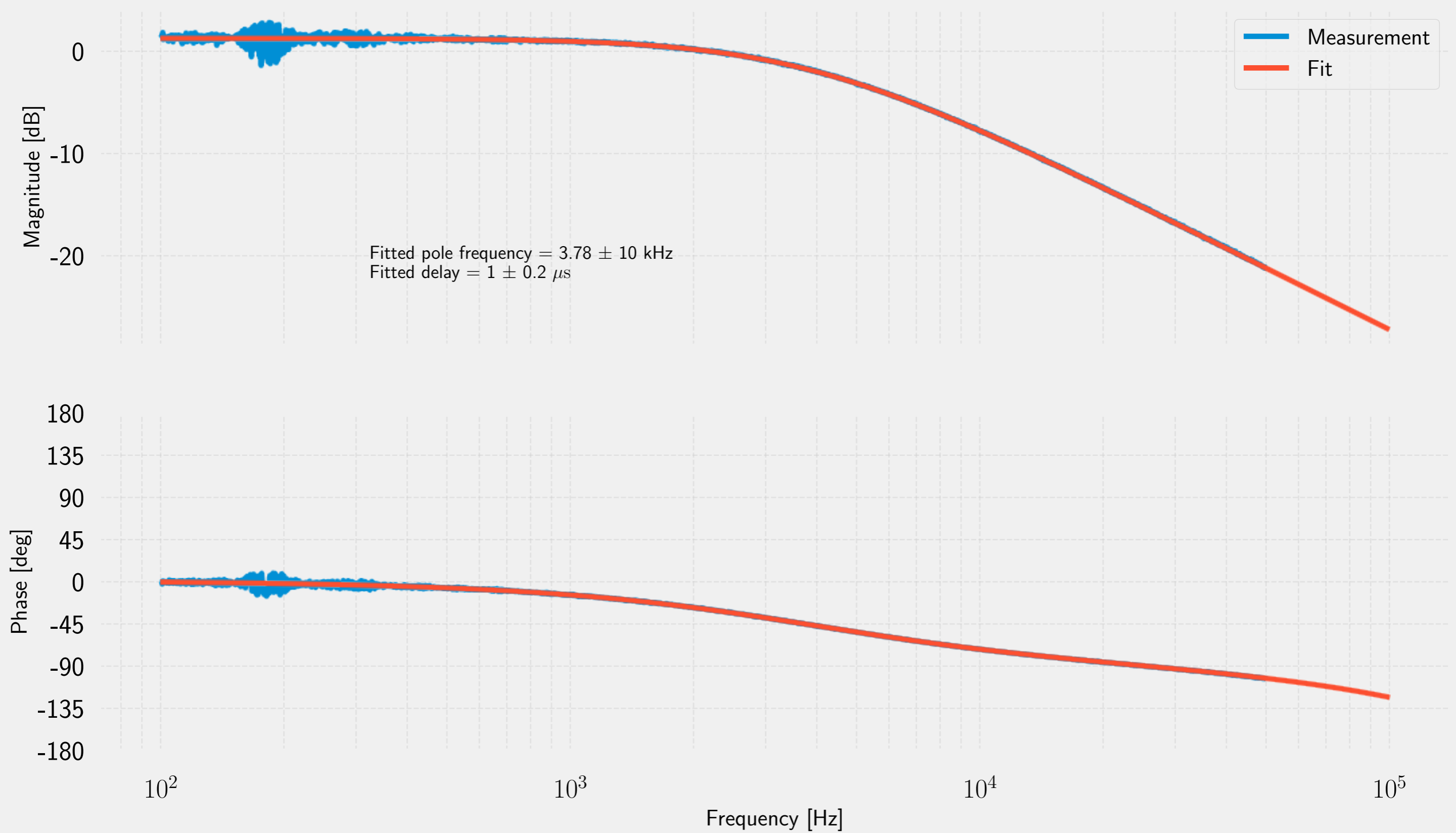
40m IMC cavity pole measurement
