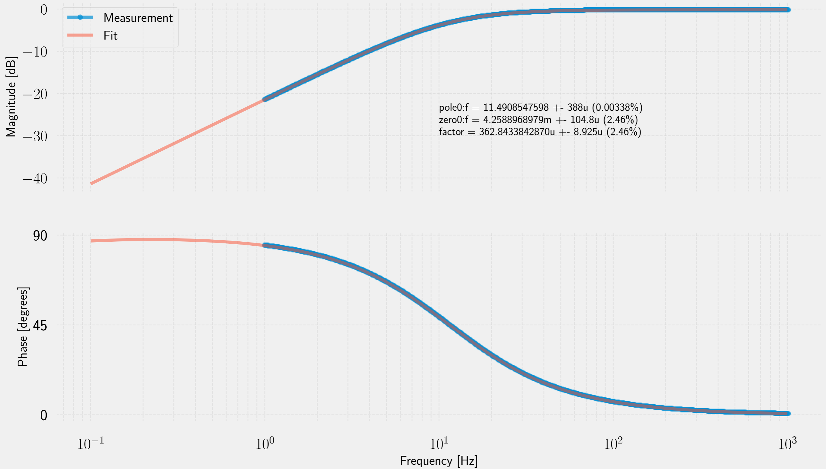
AC coupling of IMC servo IN2 (AO path)
