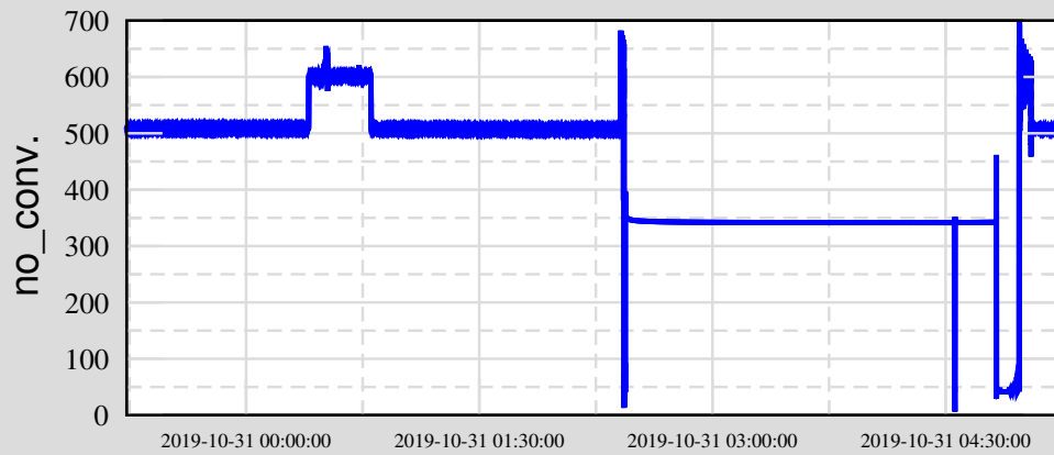
Ch 1: C1:SUS-PRM_SENSOR_LL
