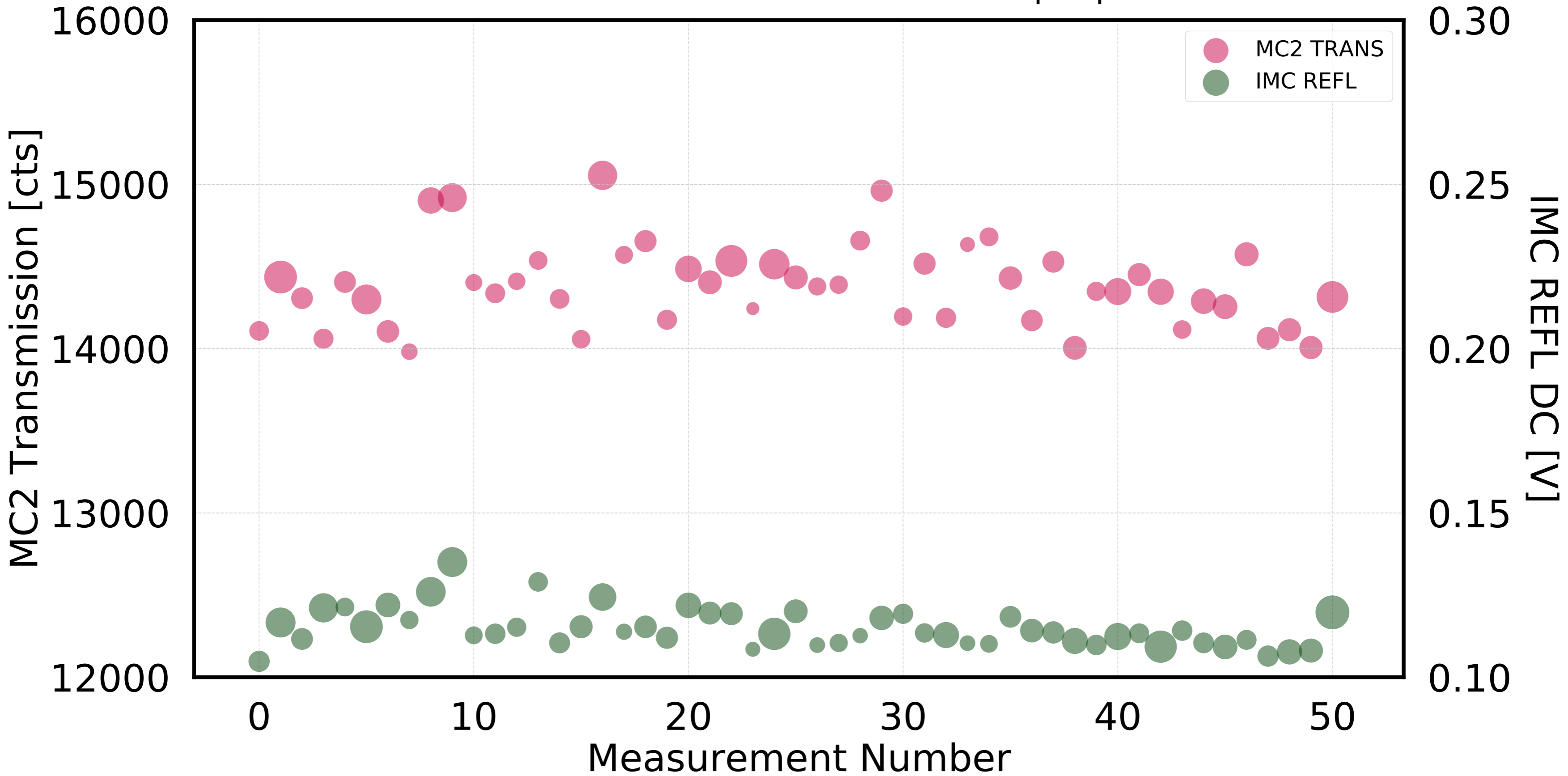
Variation of IMC REFL and MC2 TRANS for different spot positions on MC2
