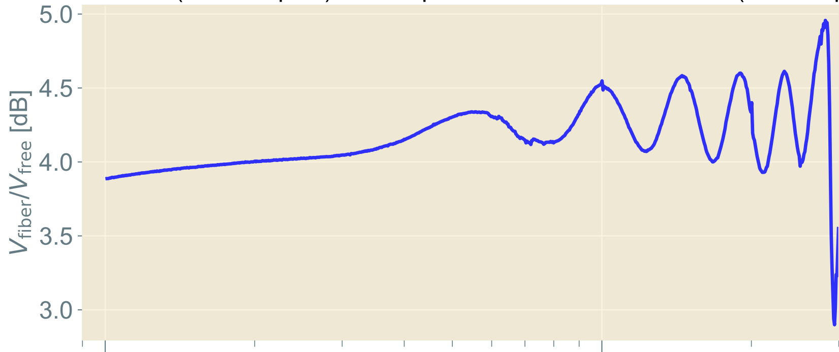
NewFocus 1611 (fiber-coupled) RF Response Relative to Reference (free-coupled) PD
