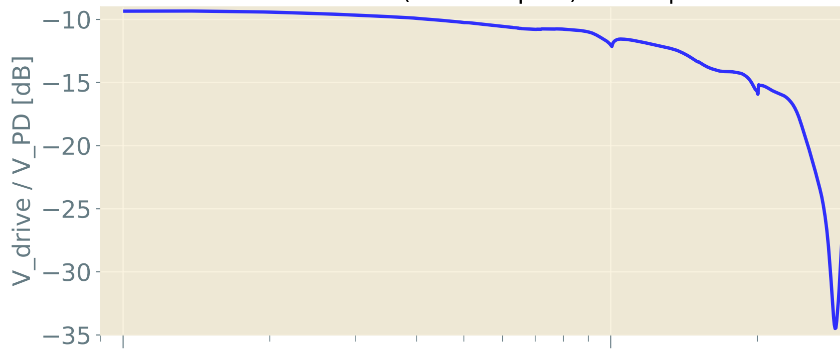
NewFocus 1611 (fiber-coupled) RF Response
