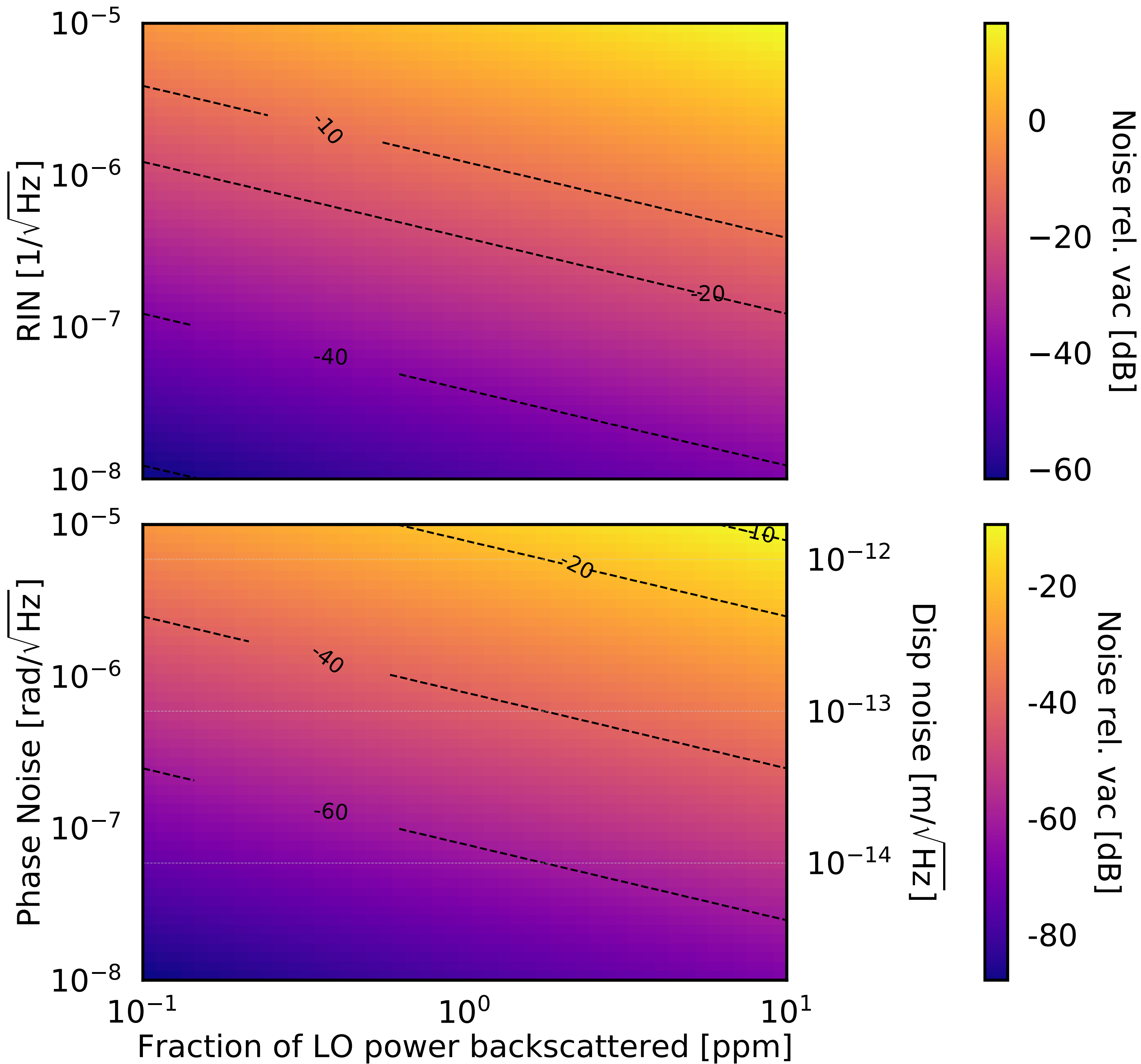
Backscatter field noise relative to vacuum, assuming P_{LO} = 50.0 mW
