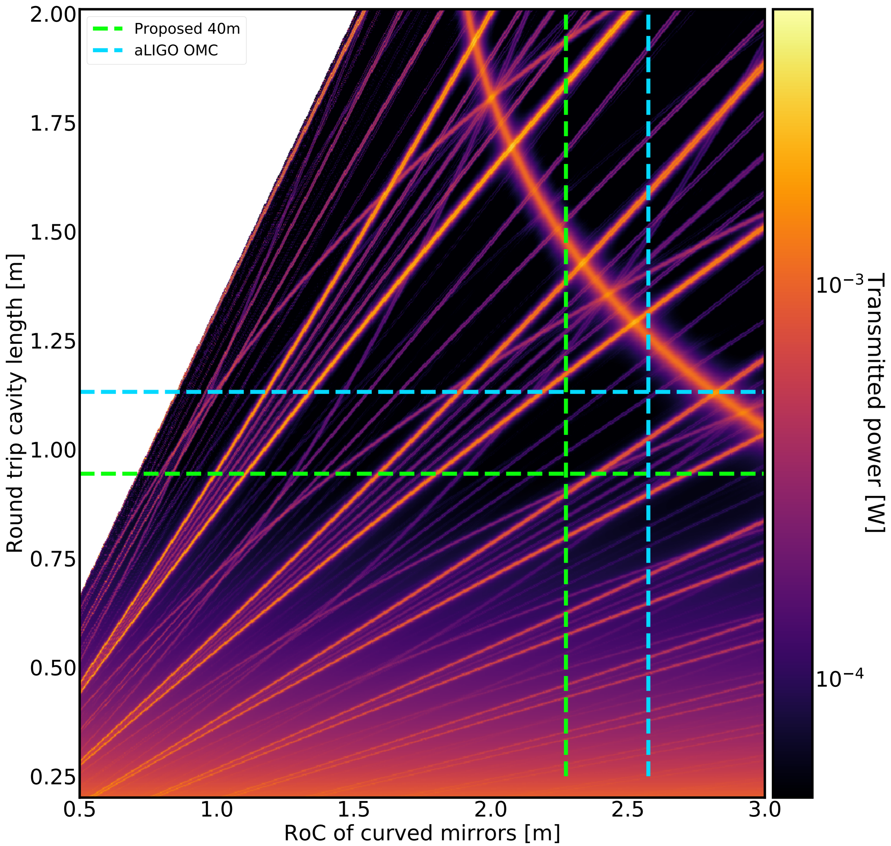
Choosing cavity geometry for 40m OMC
