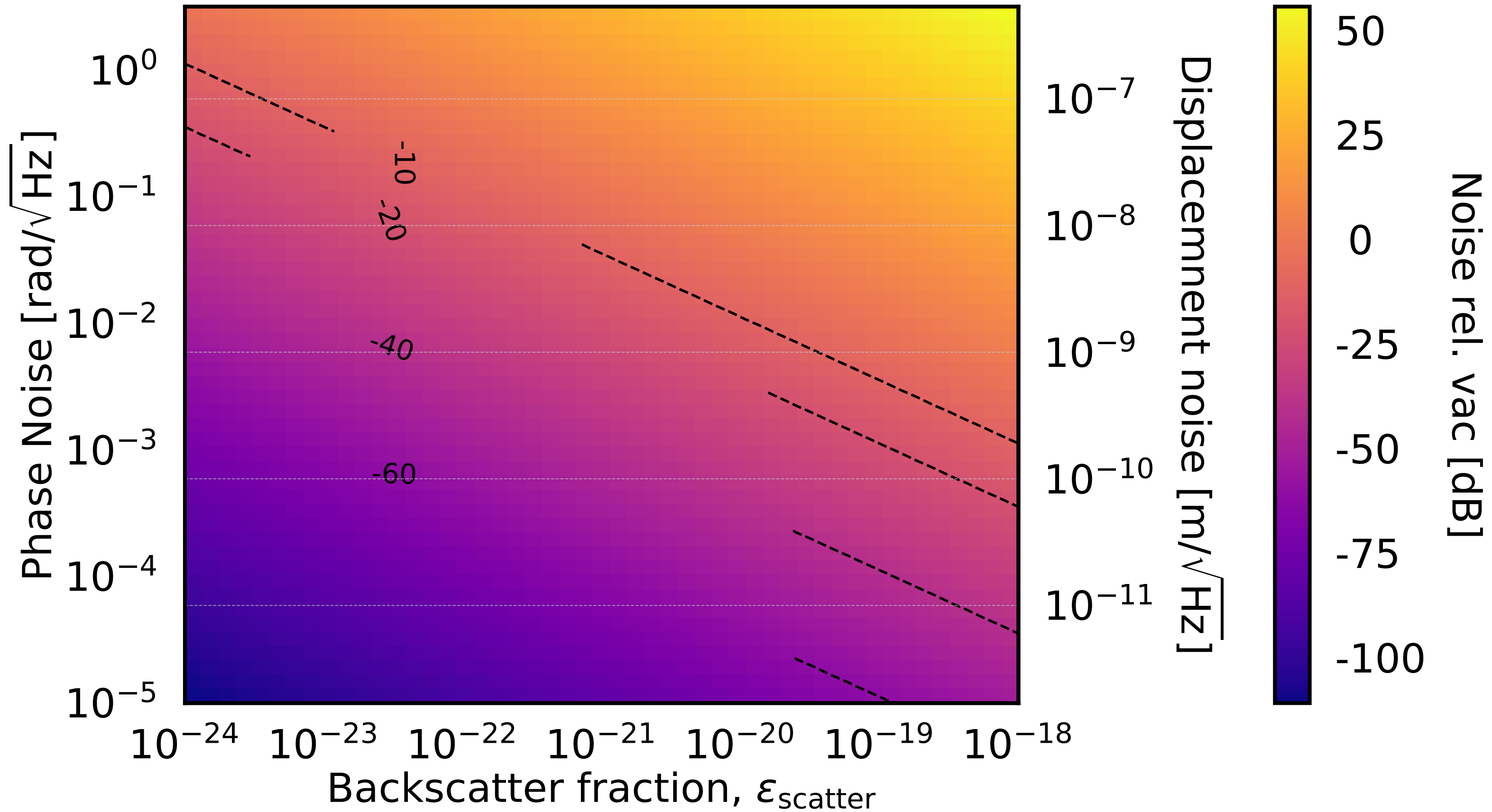
Noise due to direct backscatter onto DCPDs from 60.0 kW in arm cavity
