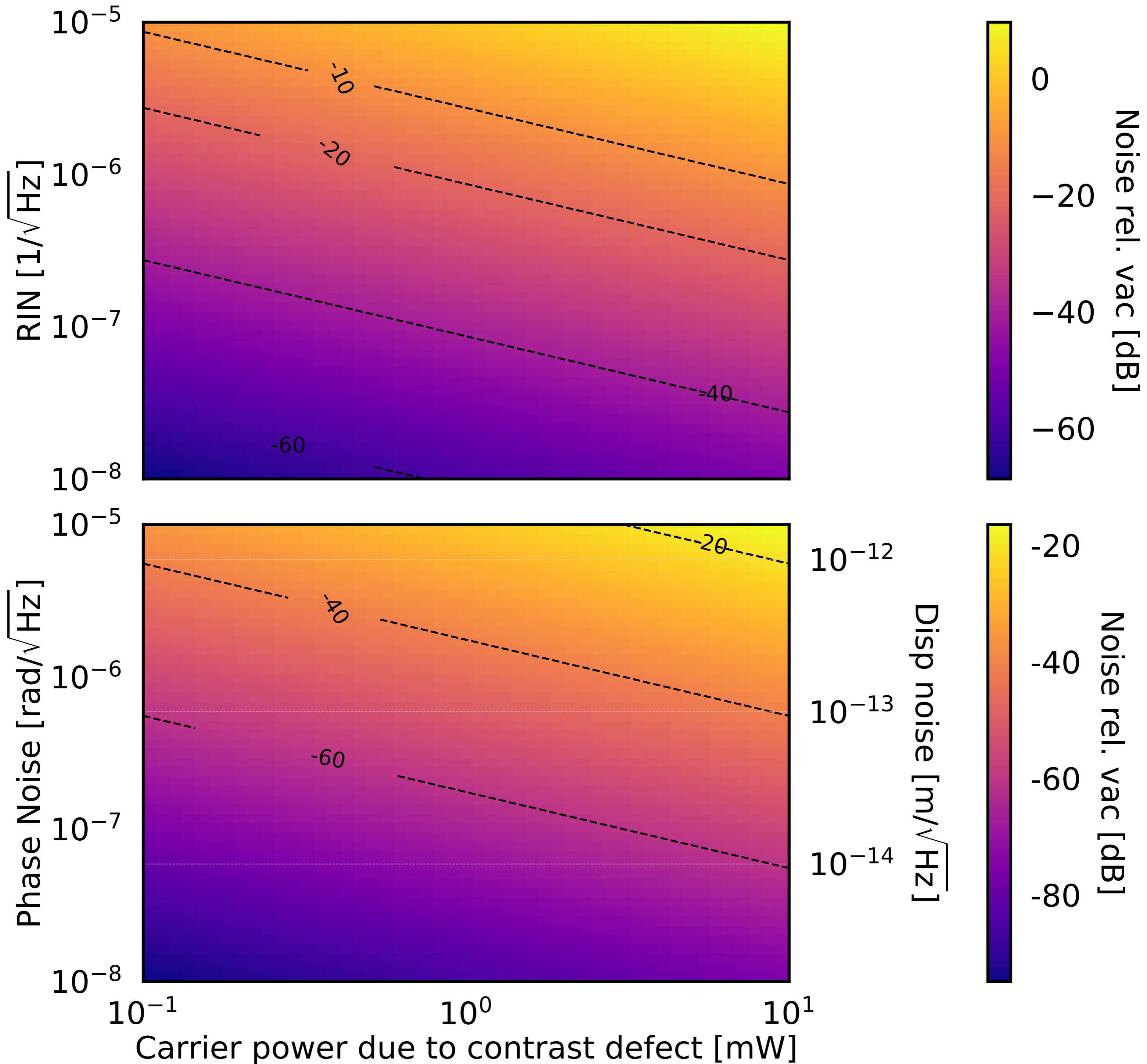
Backscatter field noise relative to vacuum for \epsilon_{BS} = 10 ppm
