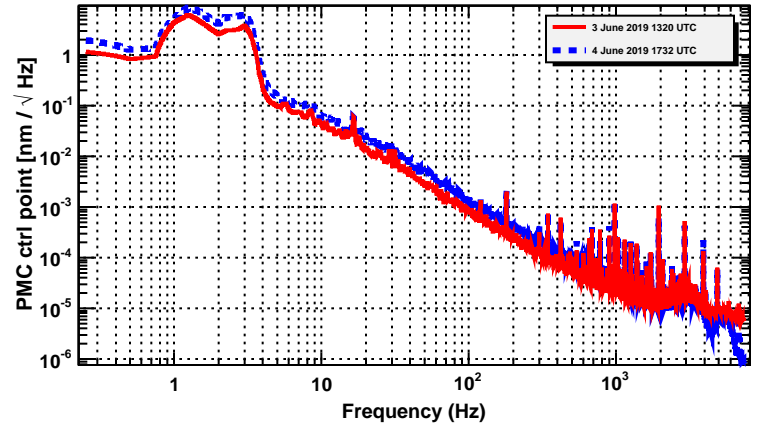
Power spectrum
