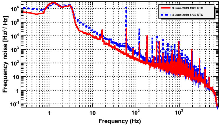
Power spectrum
