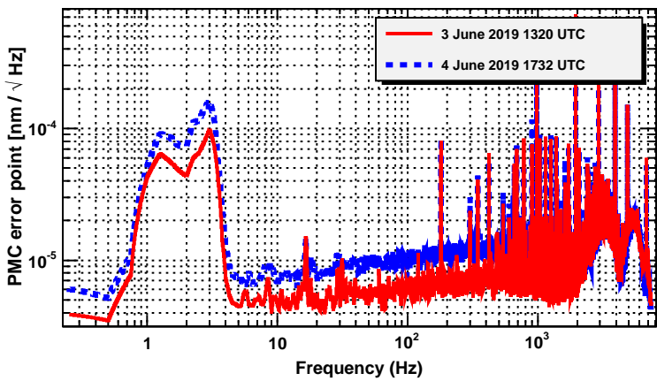
Power spectrum
