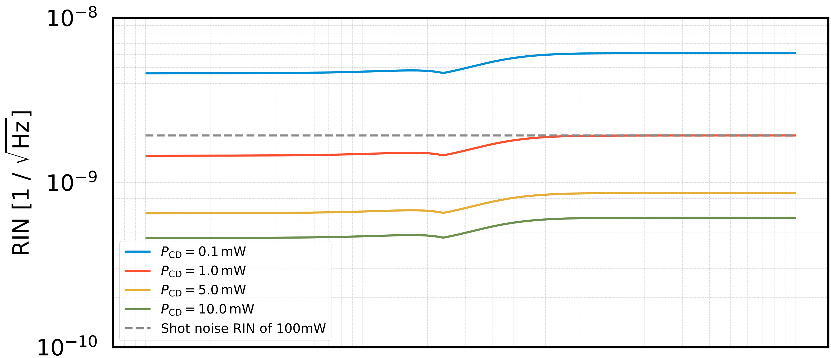
LO requirements for the 40m Ponderomotive Squeezing BHD readout
