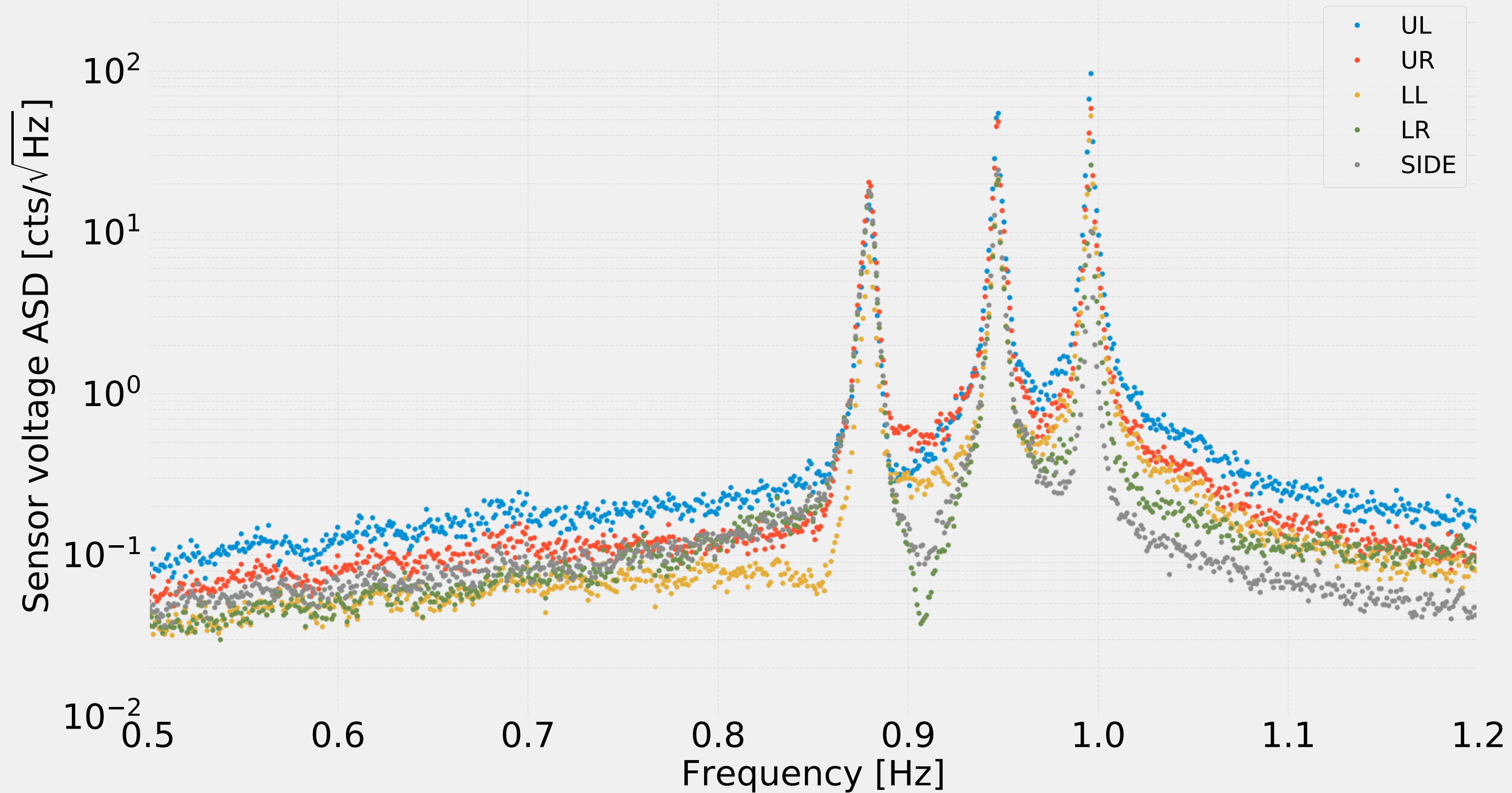
ETMY Sensor voltage spectra from 15 May 2019 1746 PDT for 15000 seconds
