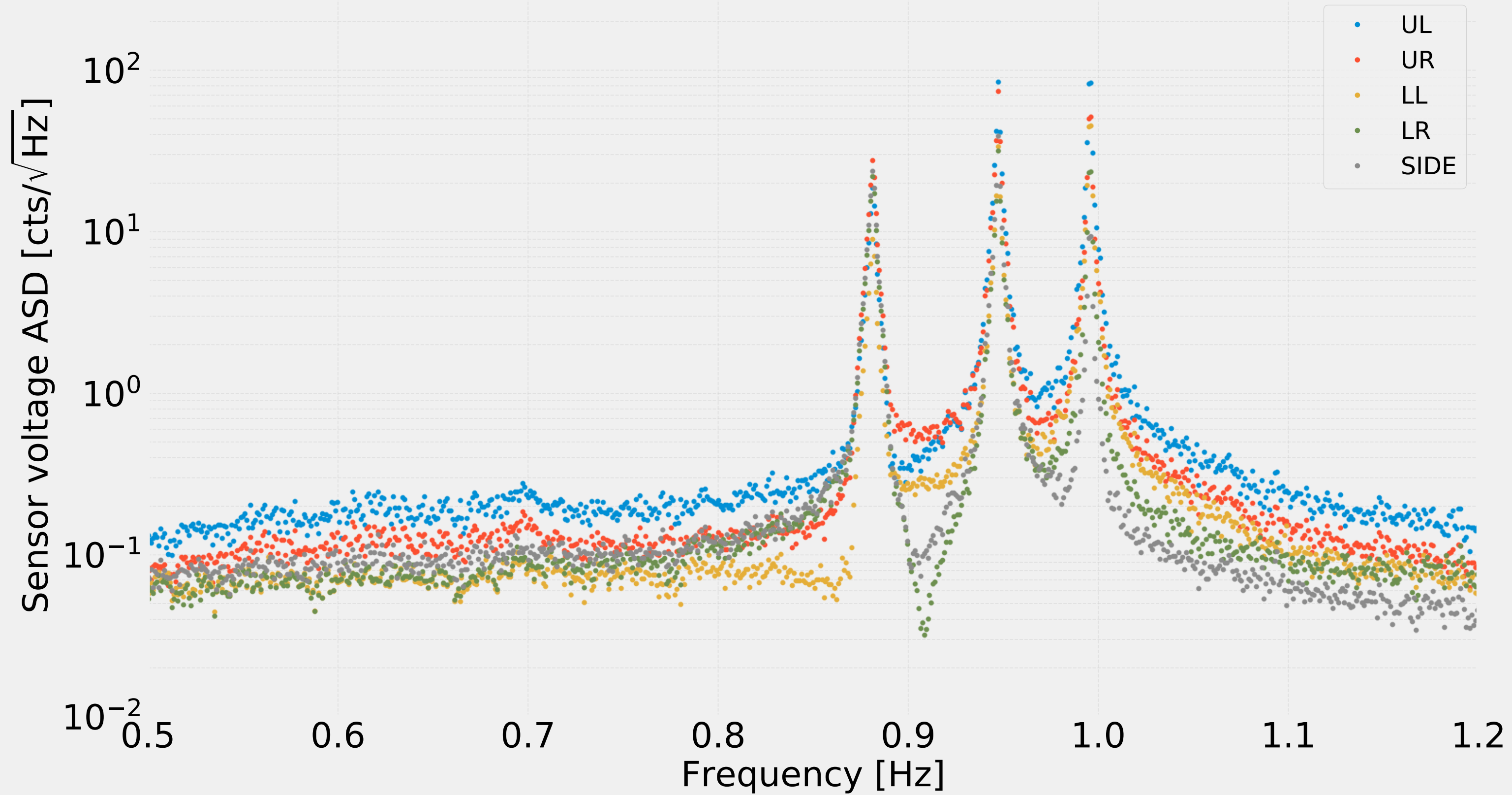
ETMY Sensor voltage spectra from 14 May 2019 1838 PDT for 15000 seconds
