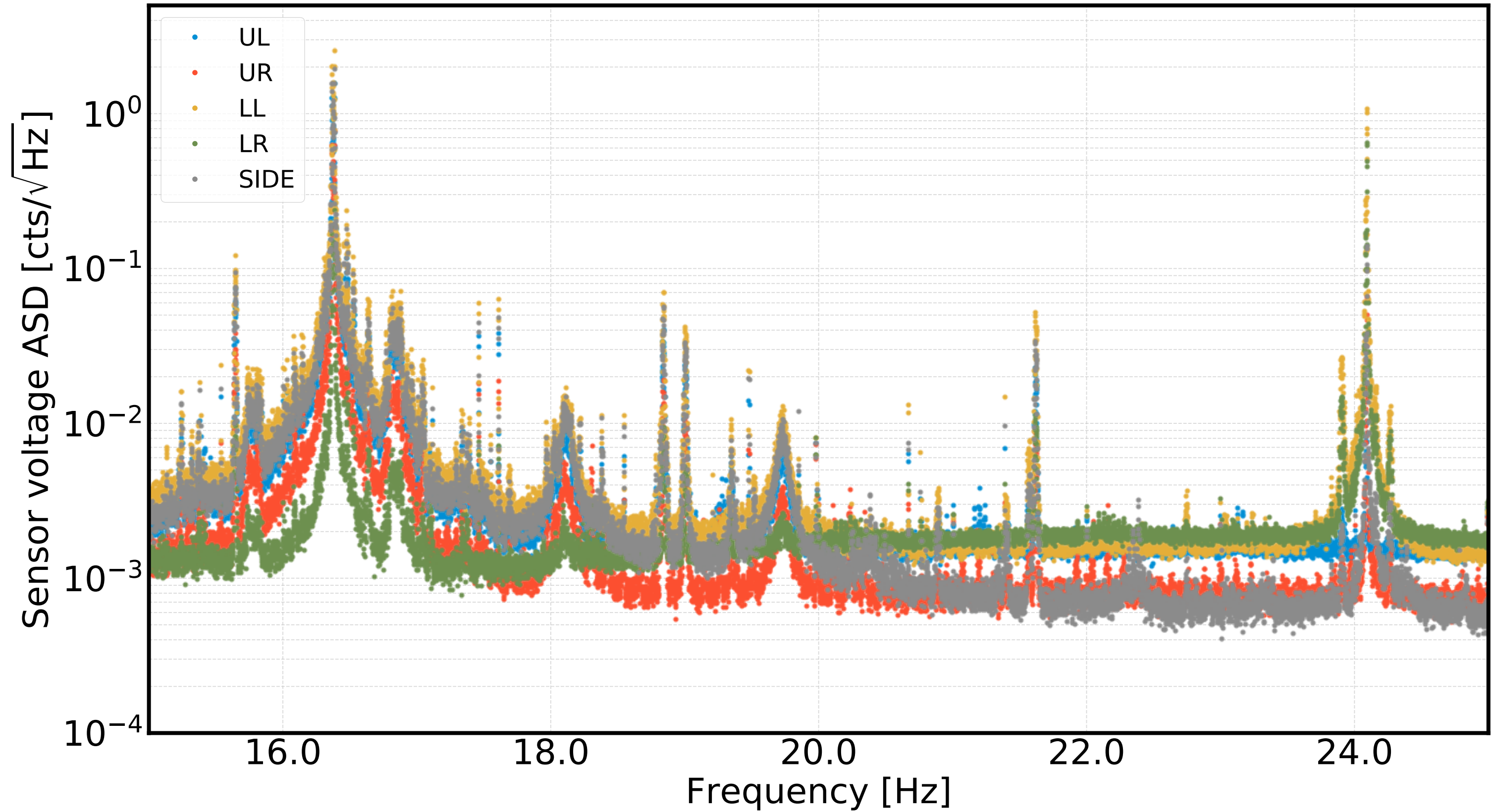
ETMX Sensor voltage spectra from 27 Feb 2019 2130 PST for 15000 seconds
