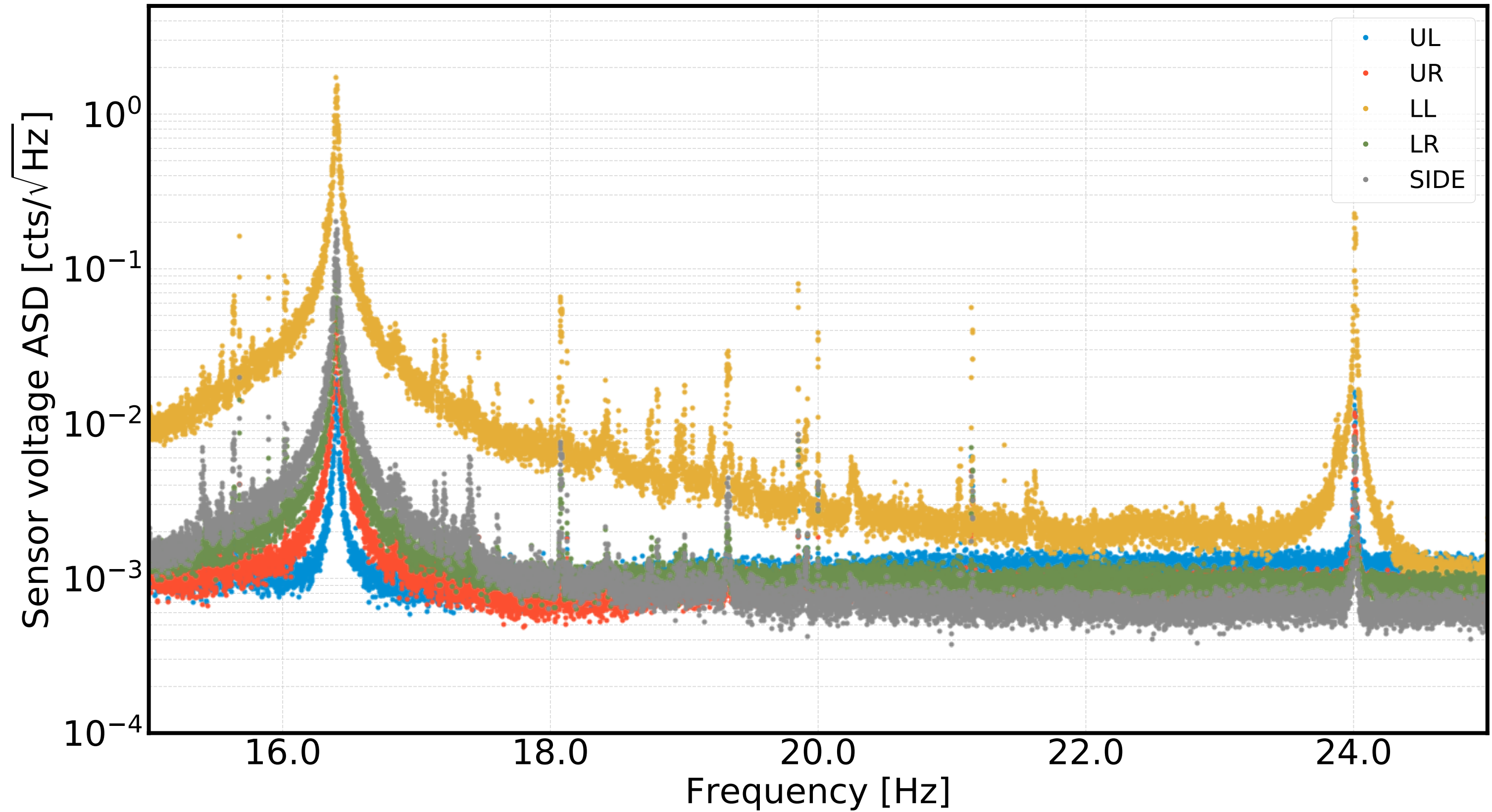
ETMY Sensor voltage spectra from 17 Apr 2019 1655 PDT for 15000 seconds
