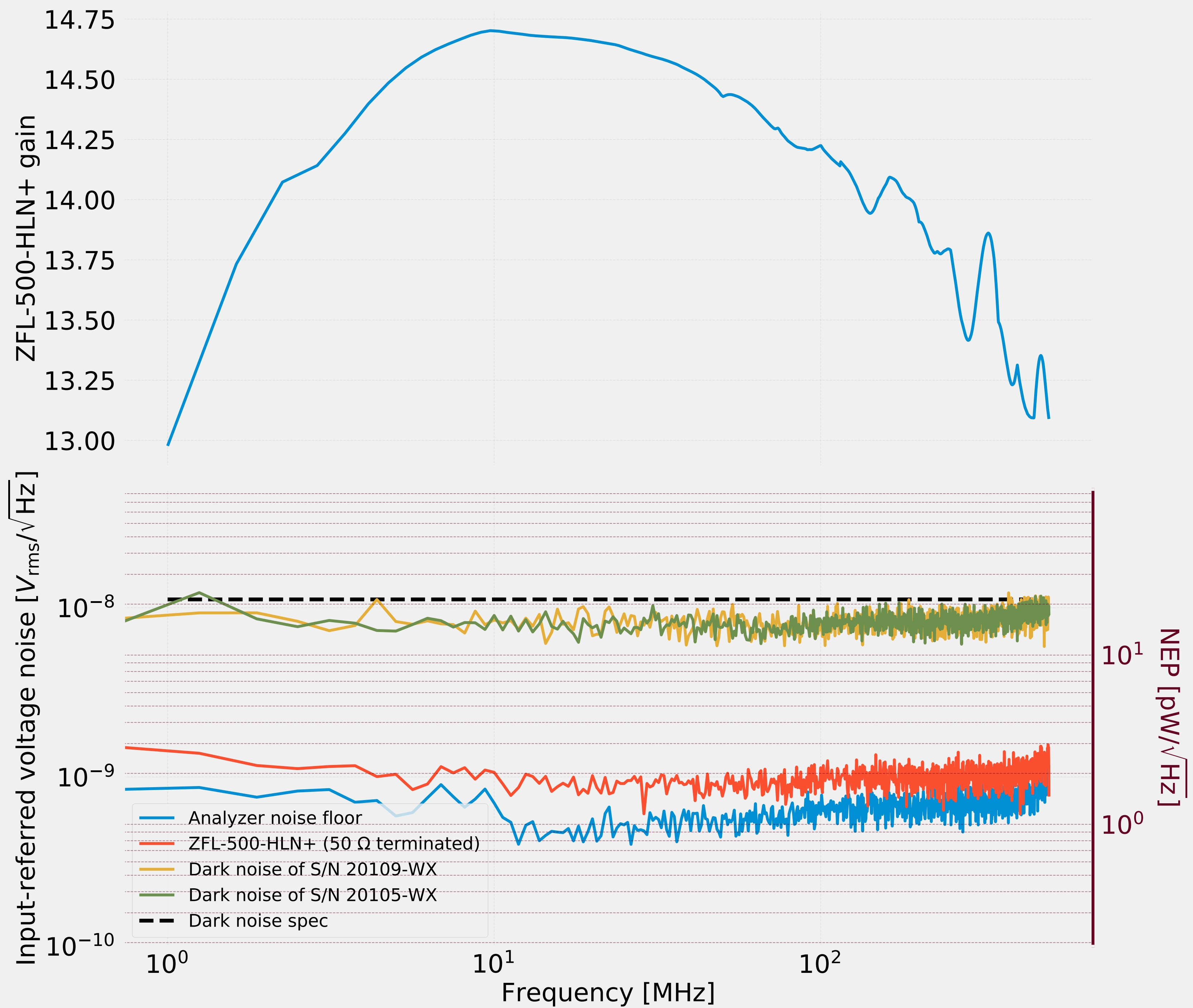
Dark noise characterization of NF1611 PDs with ZFL preamp (S/N F961501440)
