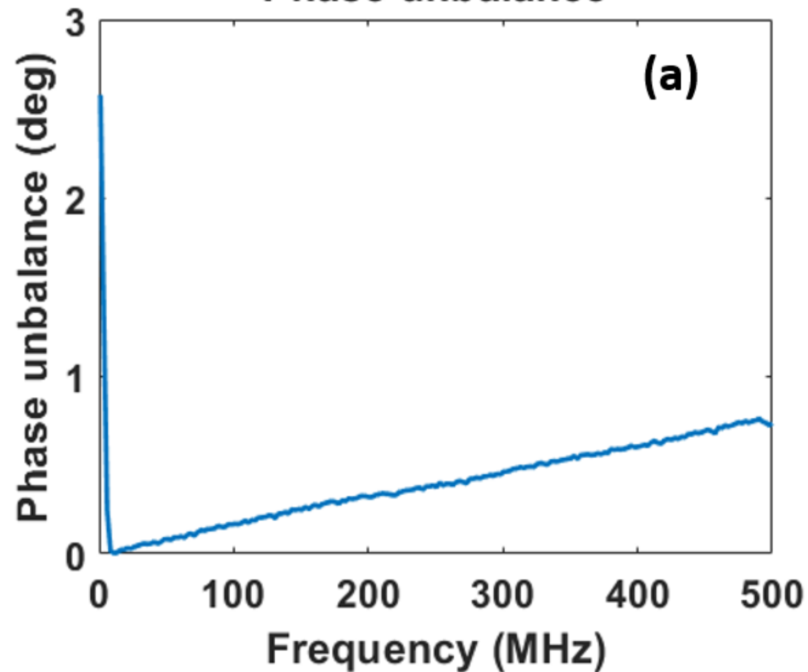
Phase unbalance
