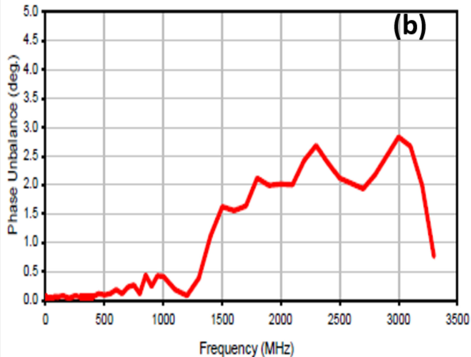
Phase Unbalance
