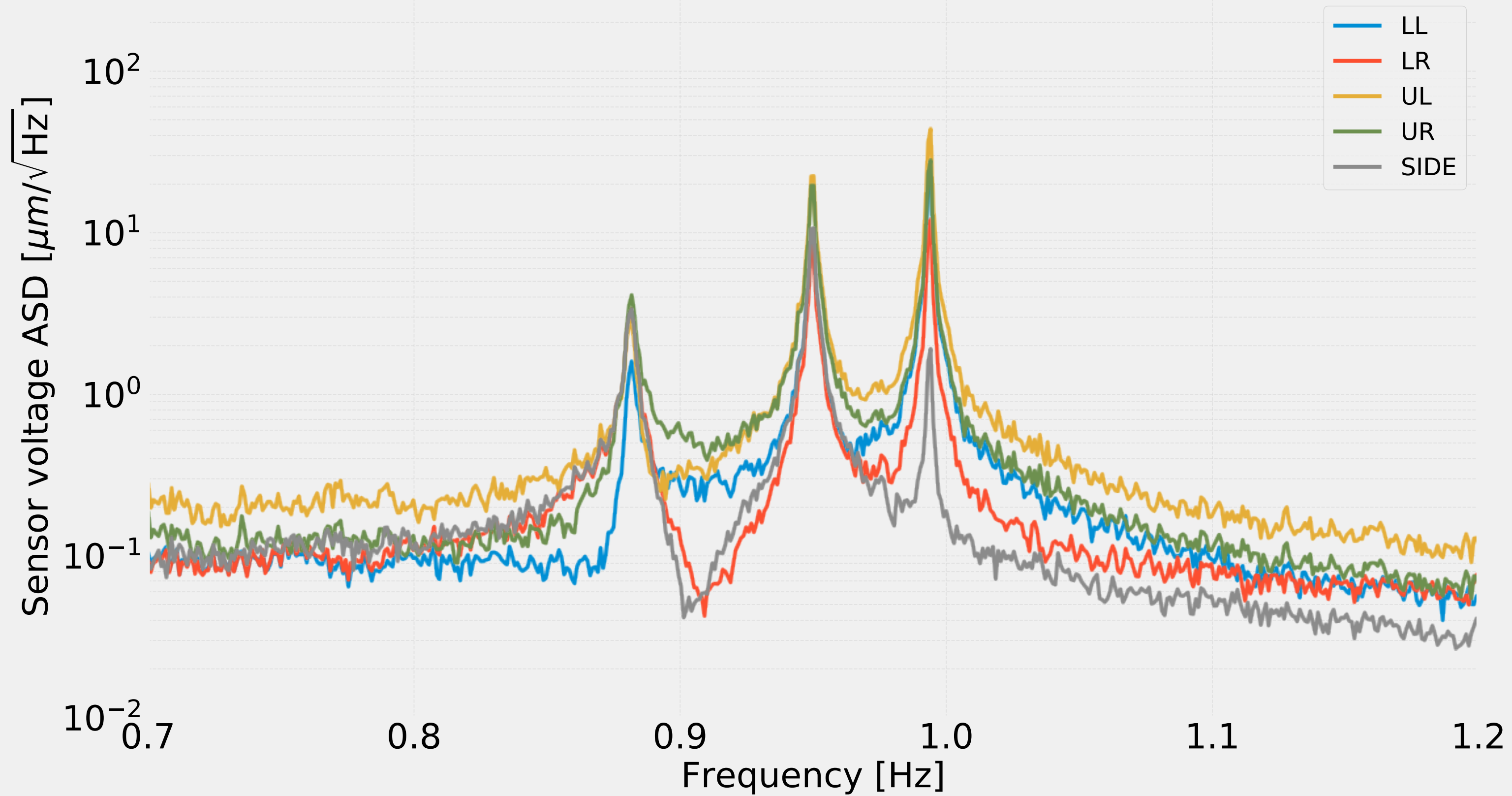
ETMY Sensor voltage spectra from 1 Feb 2019 2230 PST for 15000 seconds
