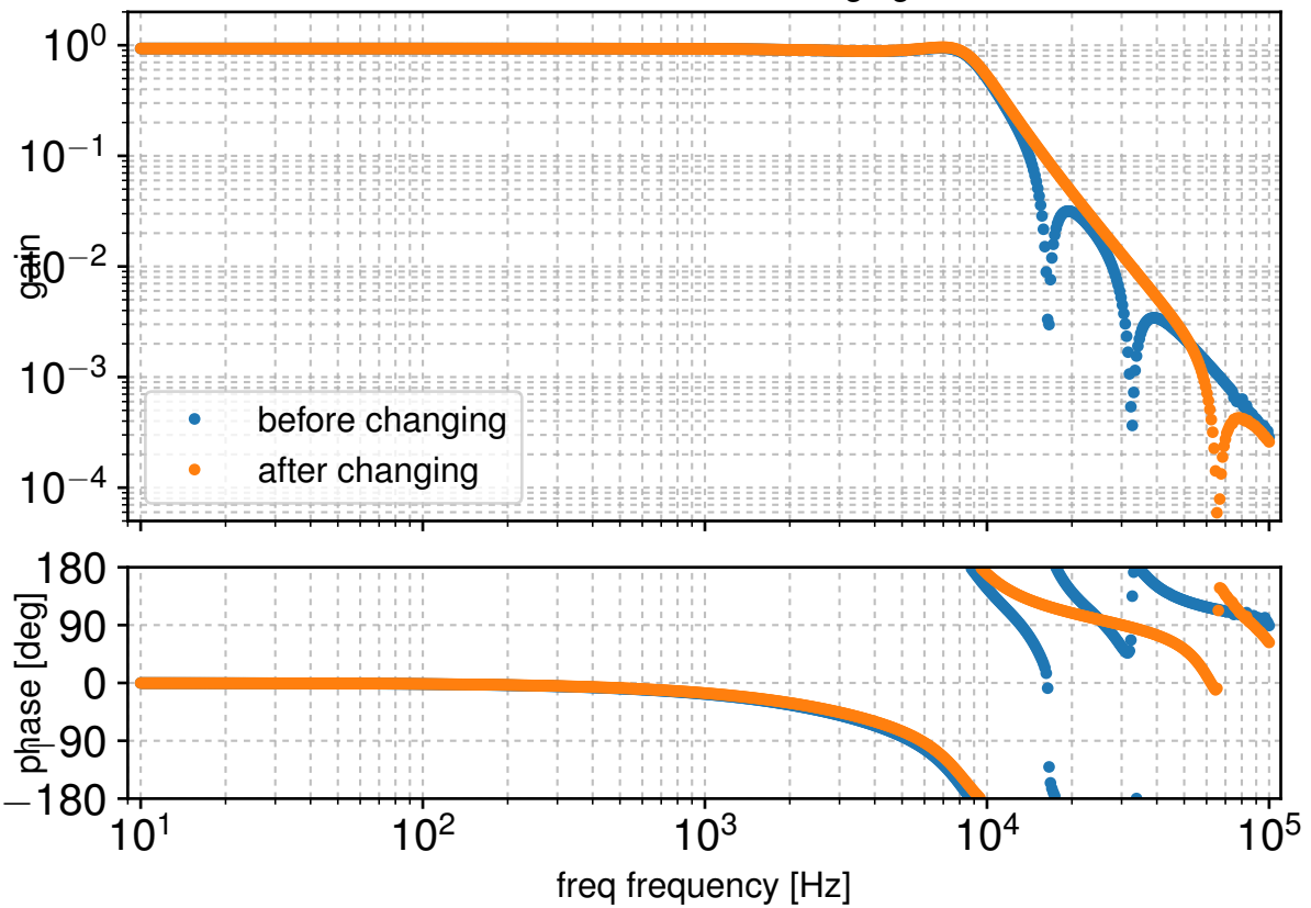
Transfer Function of Anti-Imaging board
