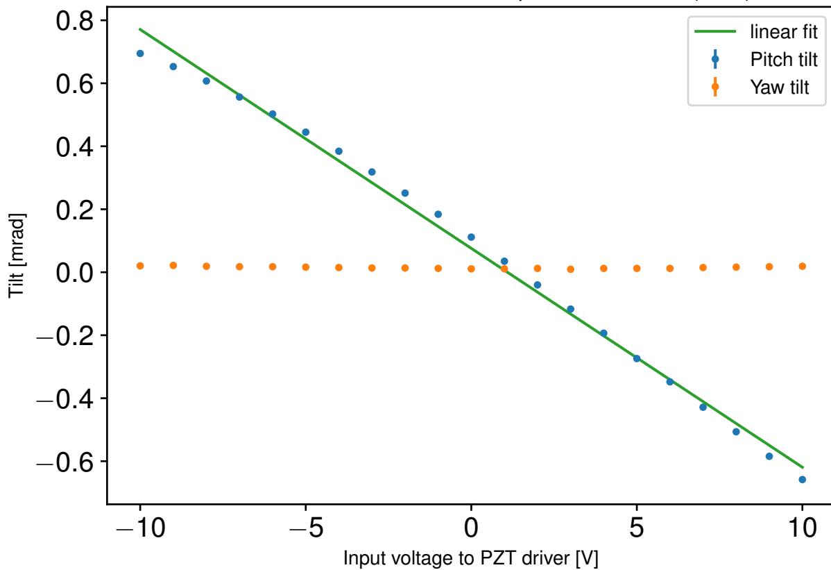
1inch PZT Mirror Calibration - Input to PZT Pitch (CH2)
