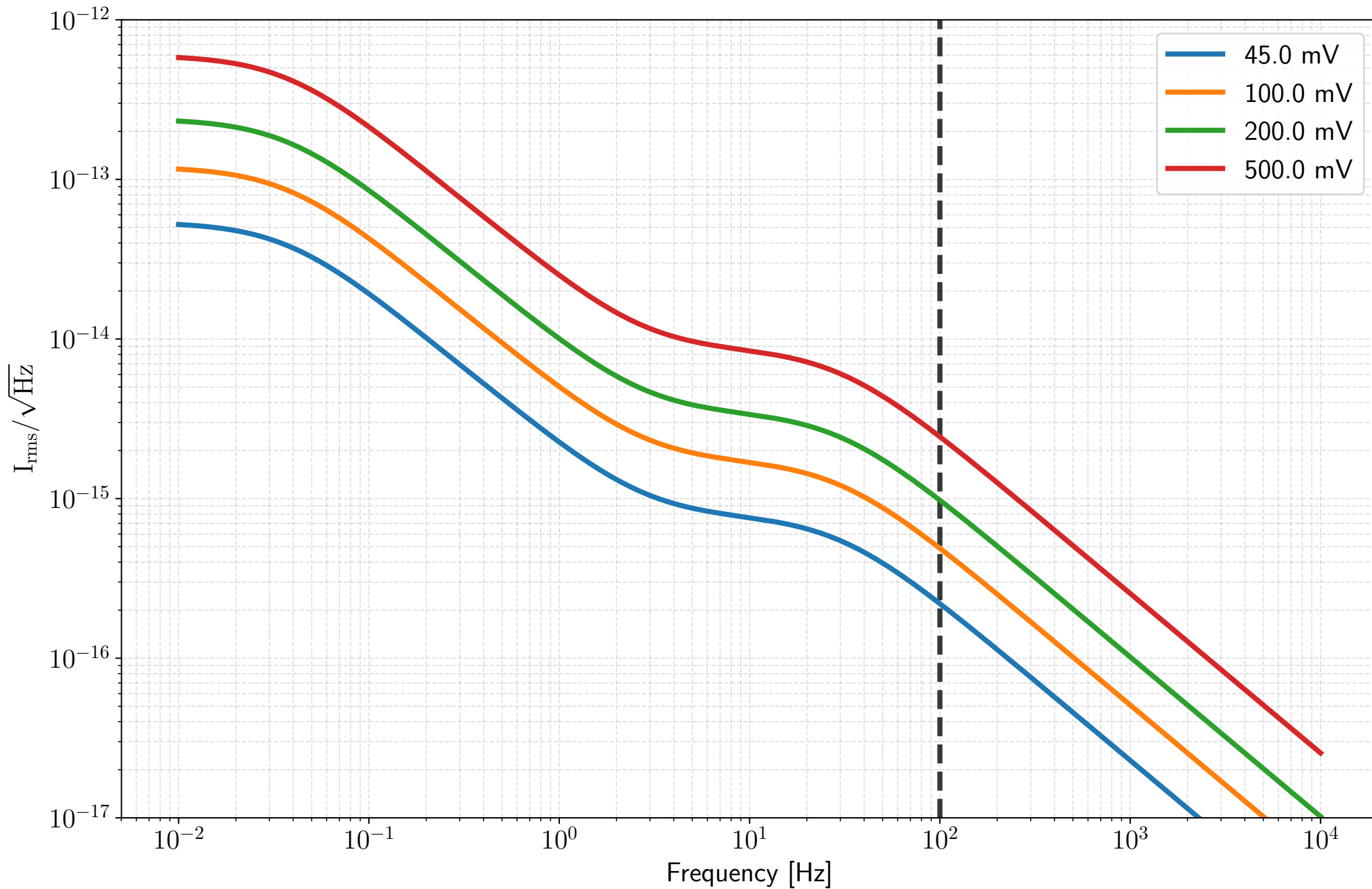
Estimated contribution of HV power supply ripple to output current noise
