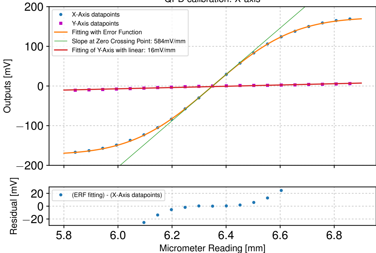
QPD calibration: X-axis
