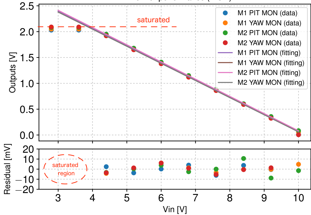
PZT driver performance (MON)
