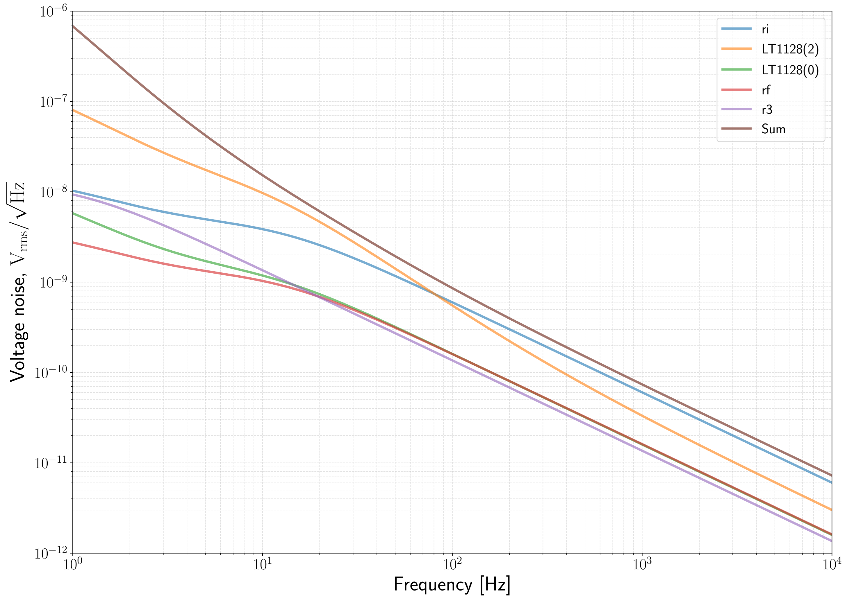
Voltage noises (before series resistor) for proposed HV bias circuit
