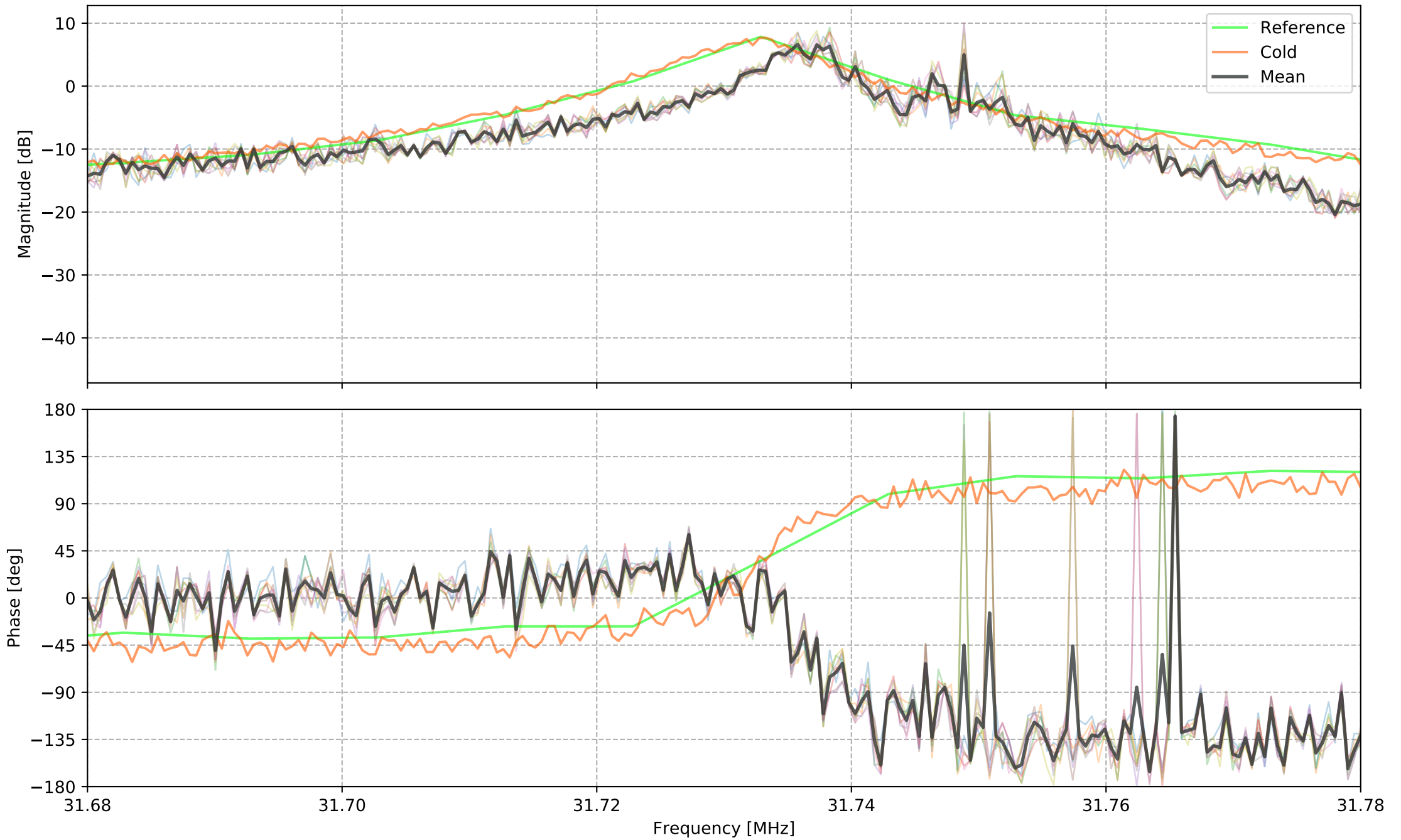
Trans/Refl scan
