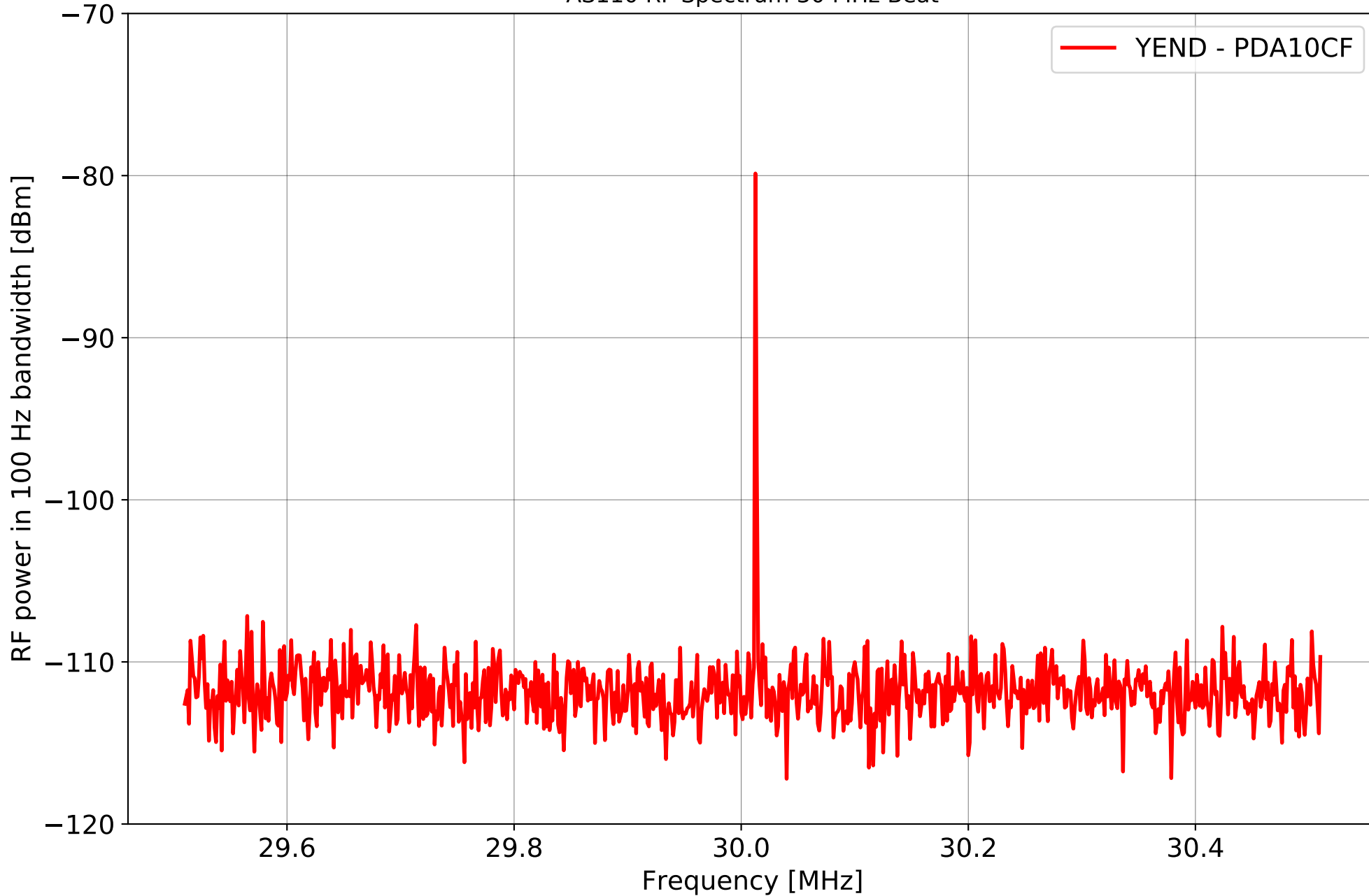
AS110 RF Spectrum 30 MHz Beat
