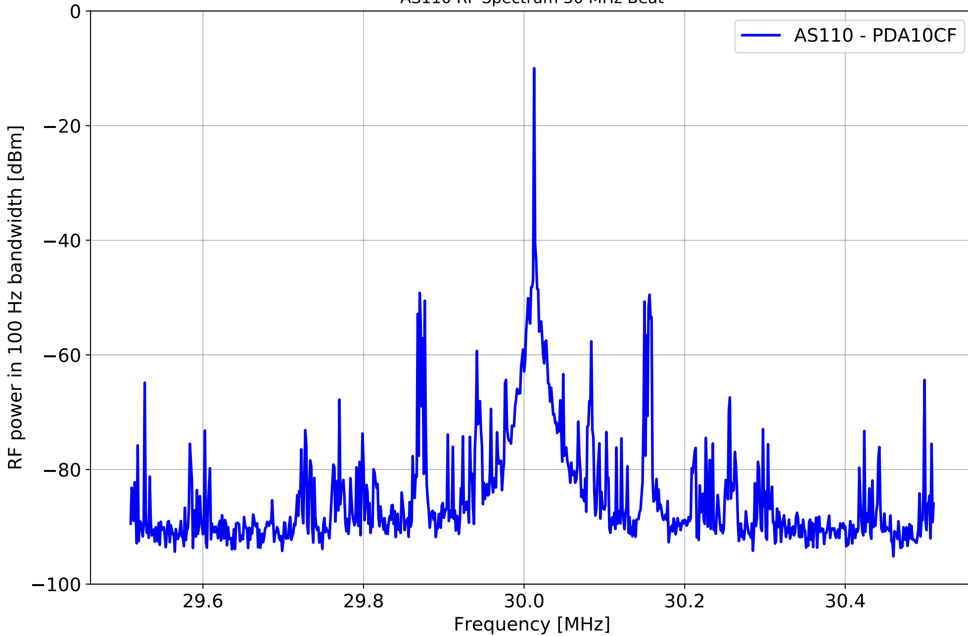
AS110 RF Spectrum 30 MHz Beat
